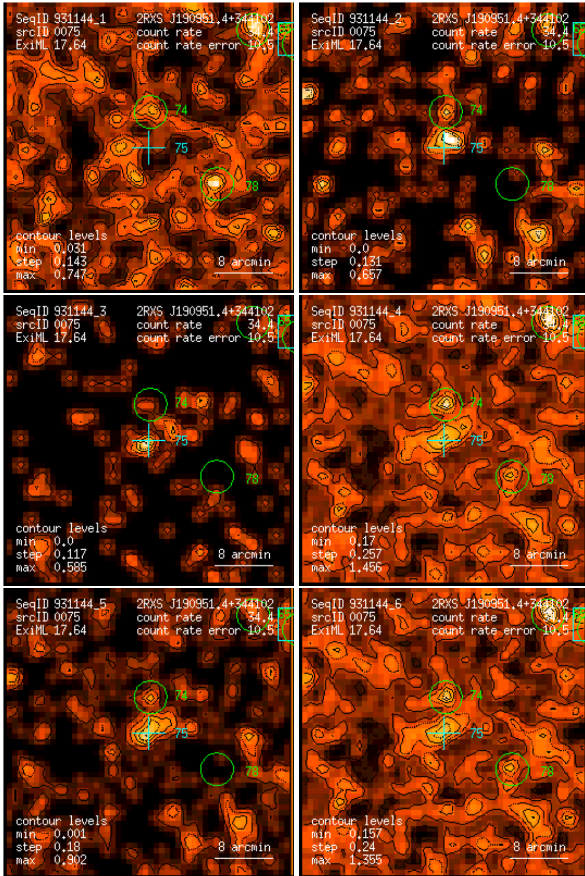
Figure 75: RASS 931144: detection 0075: band rate images, Gaussian filter: (1) PSPC channels 11 – 41, (2) 52 – 90, (3) 91 – 201, (4) 11 – 235, (5) 52 – 201, (6) 11 – 201. Broad band rates in counts/ks. Band rate contour levels in counts/ks/arcmin 2 .
