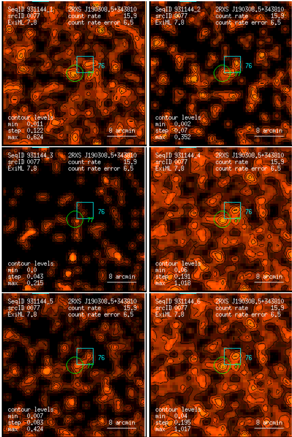
Figure 77: RASS 931144: detection 0077: band rate images, Gaussian filter: (1) PSPC channels 11 – 41, (2) 52 – 90, (3) 91 – 201, (4) 11 – 235, (5) 52 – 201, (6) 11 – 201. Broad band rates in counts/ks. Band rate contour levels in counts/ks/arcmin 2 .
