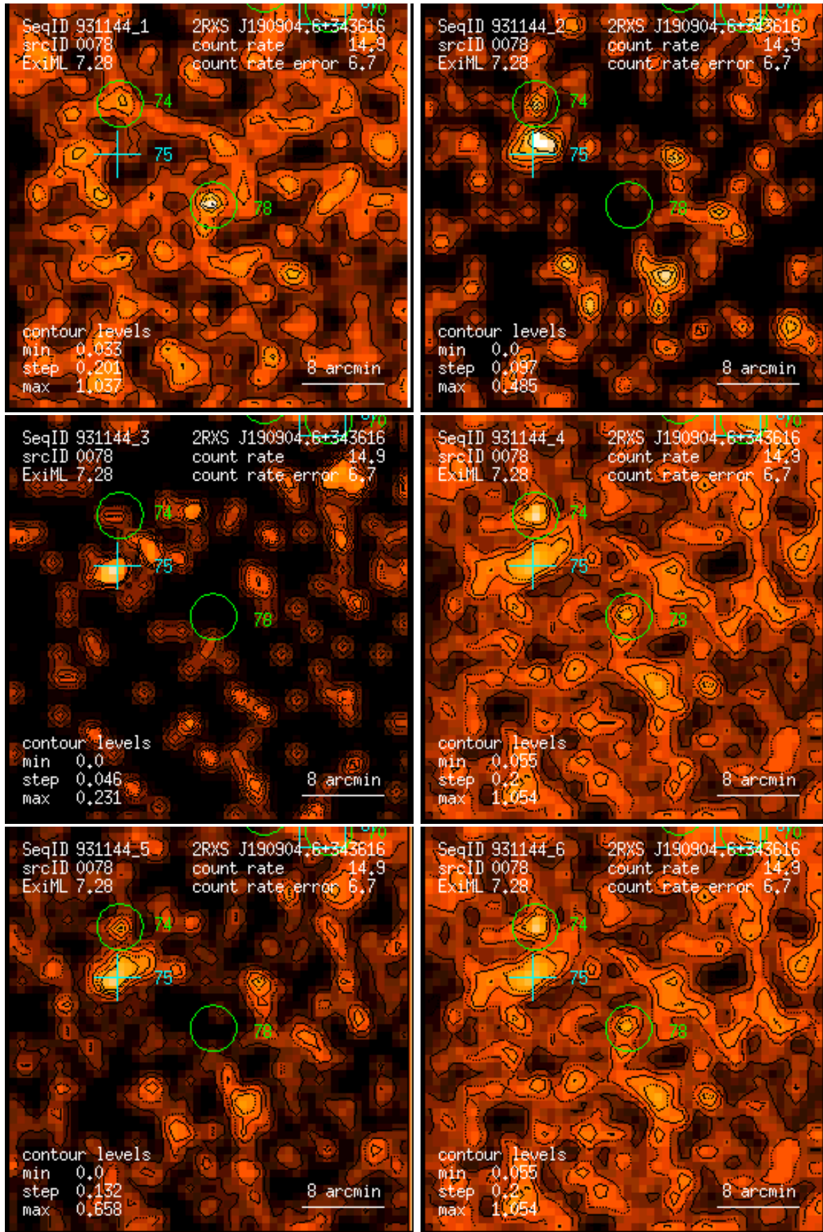
Figure 78: RASS 931144: detection 0078: band rate images, Gaussian filter: (1) PSPC channels 11 – 41, (2) 52 – 90, (3) 91 – 201, (4) 11 – 235, (5) 52 – 201, (6) 11 – 201. Broad band rates in counts/ks. Band rate contour levels in counts/ks/arcmin 2 .
