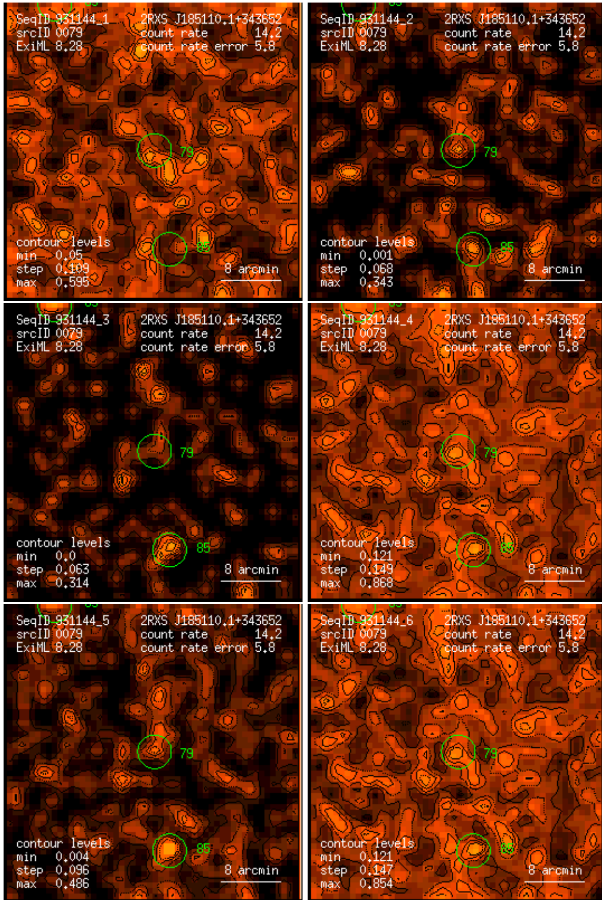
Figure 79: RASS 931144: detection 0079: band rate images, Gaussian filter: (1) PSPC channels 11 – 41, (2) 52 – 90, (3) 91 – 201, (4) 11 – 235, (5) 52 – 201, (6) 11 – 201. Broad band rates in counts/ks. Band rate contour levels in counts/ks/arcmin 2 .
