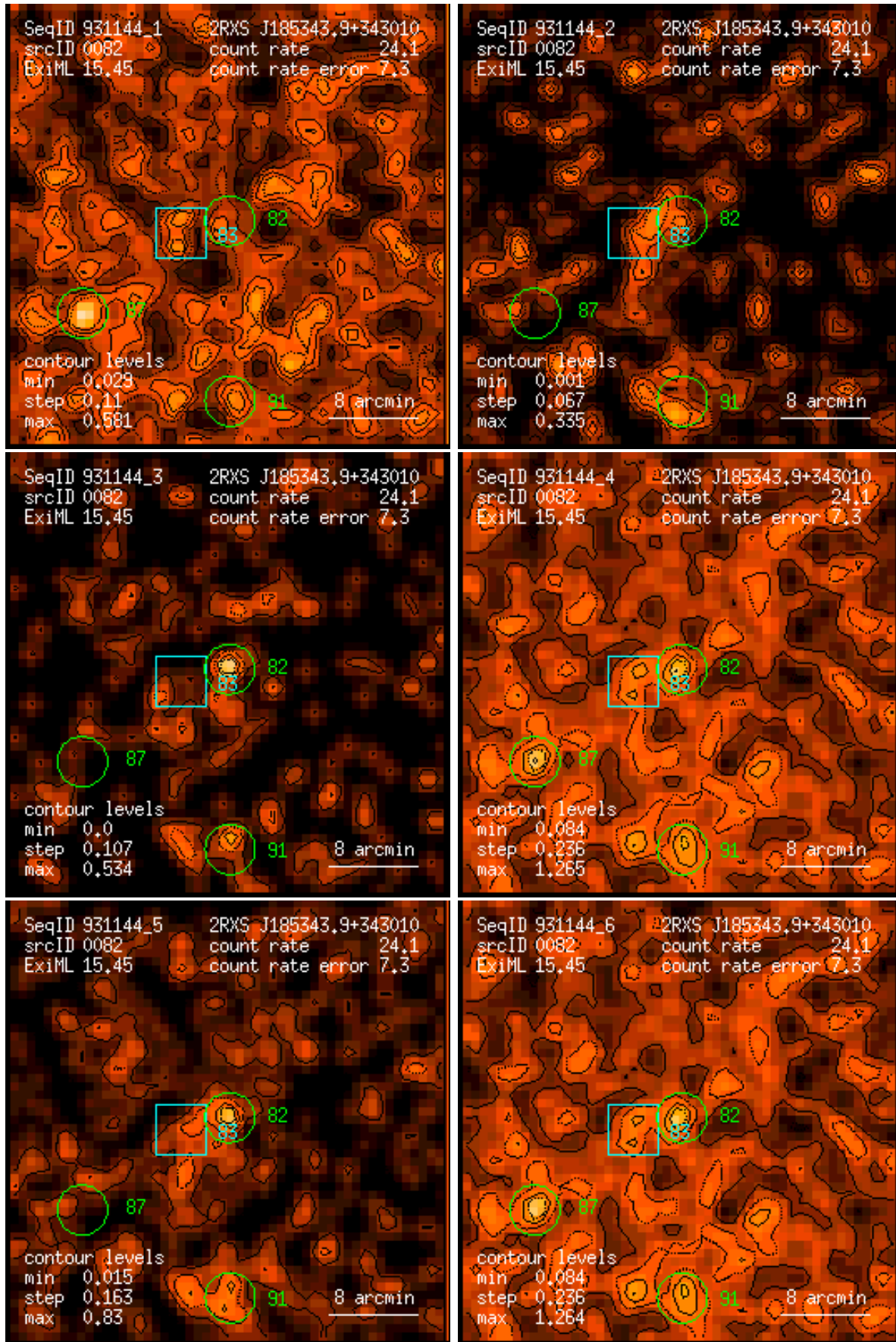
Figure 82: RASS 931144: detection 0082: band rate images, Gaussian filter: (1) PSPC channels 11 – 41, (2) 52 – 90, (3) 91 – 201, (4) 11 – 235, (5) 52 – 201, (6) 11 – 201. Broad band rates in counts/ks. Band rate contour levels in counts/ks/arcmin 2 .
