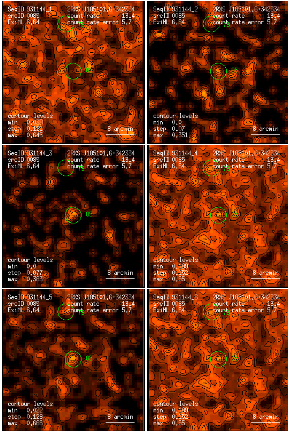
Figure 85: RASS 931144: detection 0085: band rate images, Gaussian filter: (1) PSPC channels 11 – 41, (2) 52 – 90, (3) 91 – 201, (4) 11 – 235, (5) 52 – 201, (6) 11 – 201. Broad band rates in counts/ks. Band rate contour levels in counts/ks/arcmin 2 .
