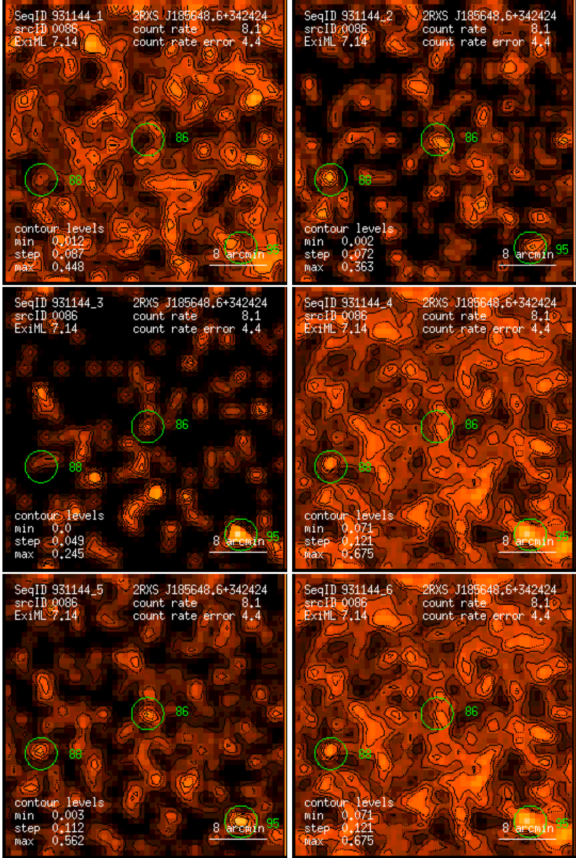
Figure 86: RASS 931144: detection 0086: band rate images, Gaussian filter: (1) PSPC channels 11 – 41, (2) 52 – 90, (3) 91 – 201, (4) 11 – 235, (5) 52 – 201, (6) 11 – 201. Broad band rates in counts/ks. Band rate contour levels in counts/ks/arcmin 2 .
