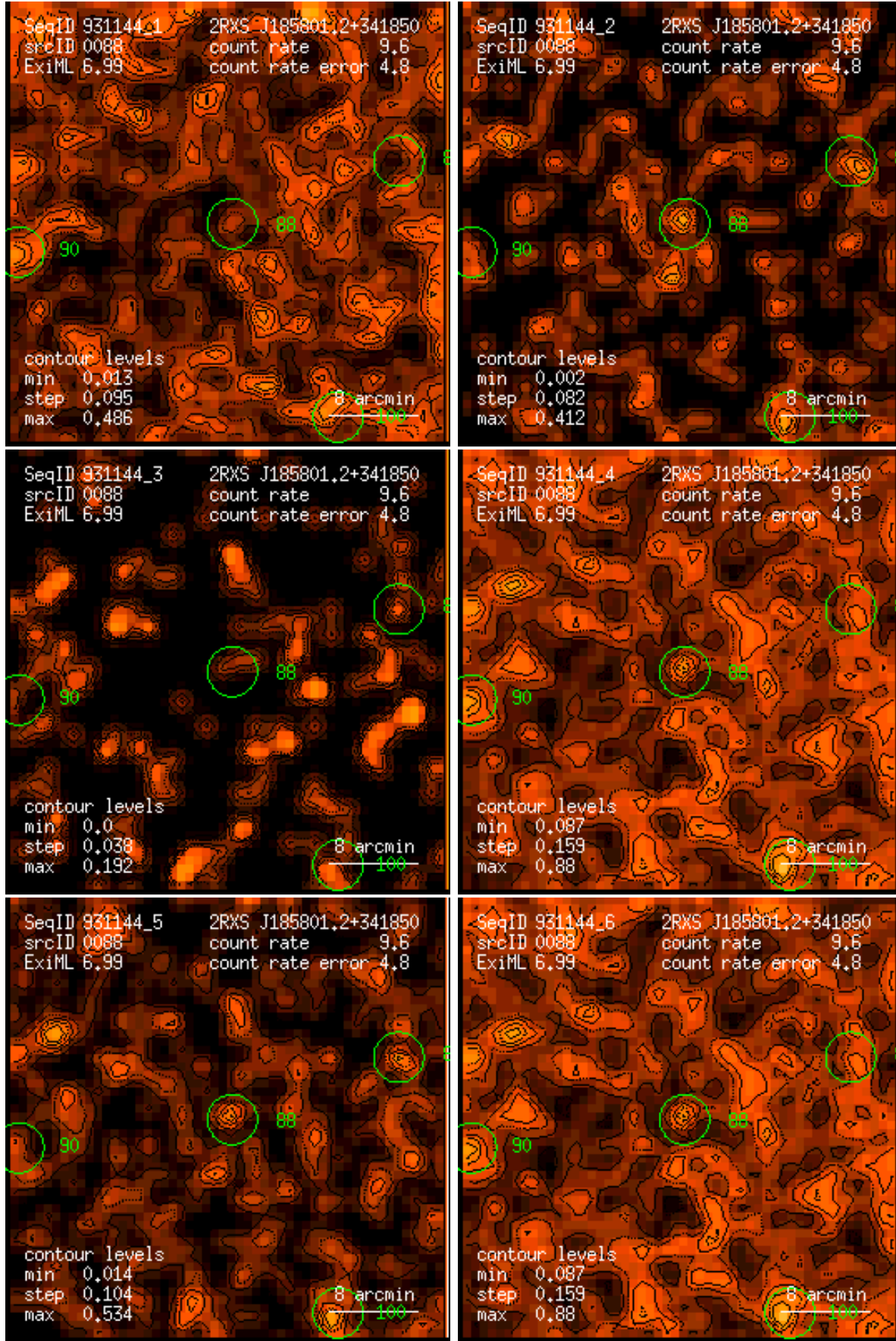
Figure 88: RASS 931144: detection 0088: band rate images, Gaussian filter: (1) PSPC channels 11 – 41, (2) 52 – 90, (3) 91 – 201, (4) 11 – 235, (5) 52 – 201, (6) 11 – 201. Broad band rates in counts/ks. Band rate contour levels in counts/ks/arcmin 2 .
