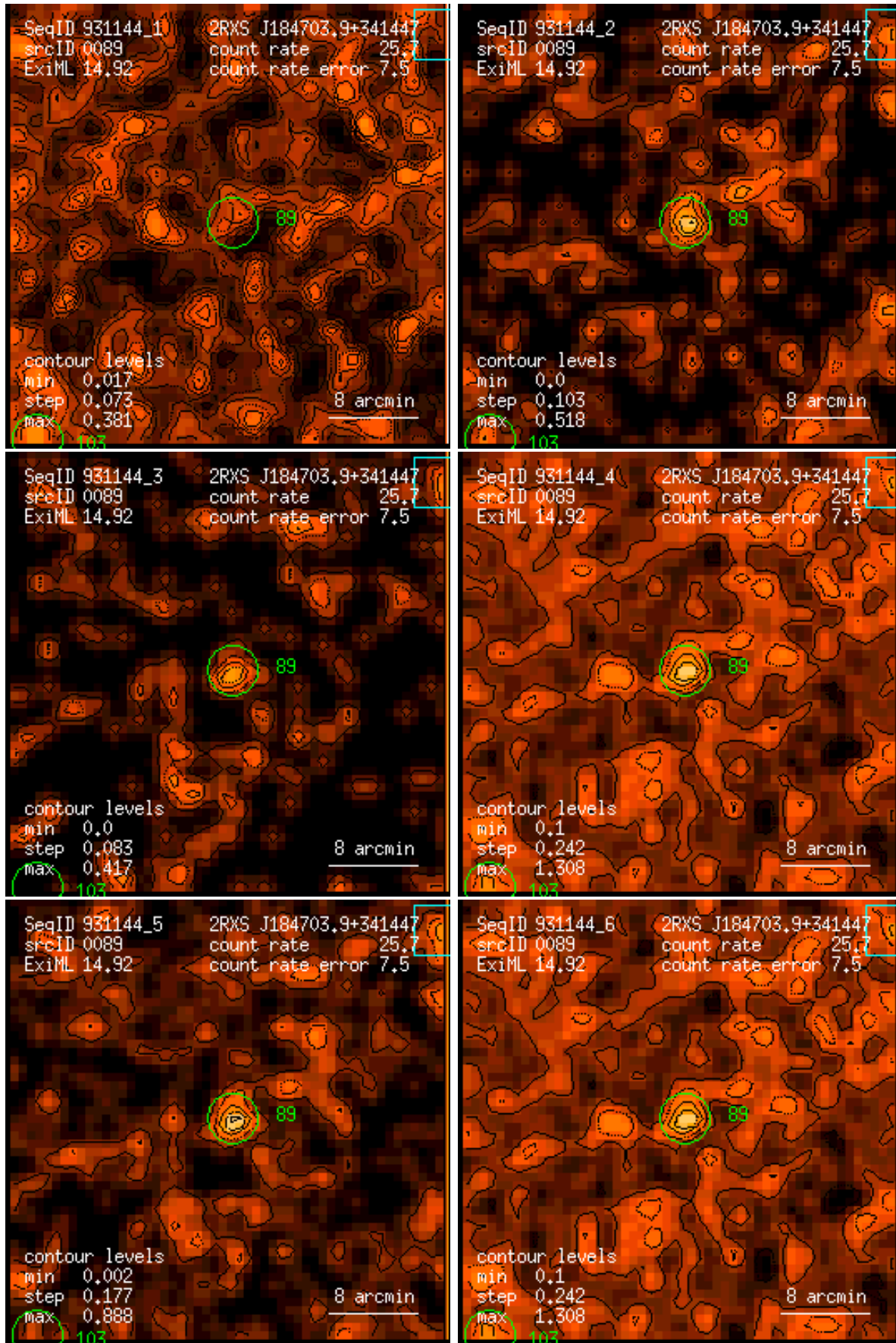
Figure 89: RASS 931144: detection 0089: band rate images, Gaussian filter: (1) PSPC channels 11 – 41, (2) 52 – 90, (3) 91 – 201, (4) 11 – 235, (5) 52 – 201, (6) 11 – 201. Broad band rates in counts/ks. Band rate contour levels in counts/ks/arcmin 2 .
