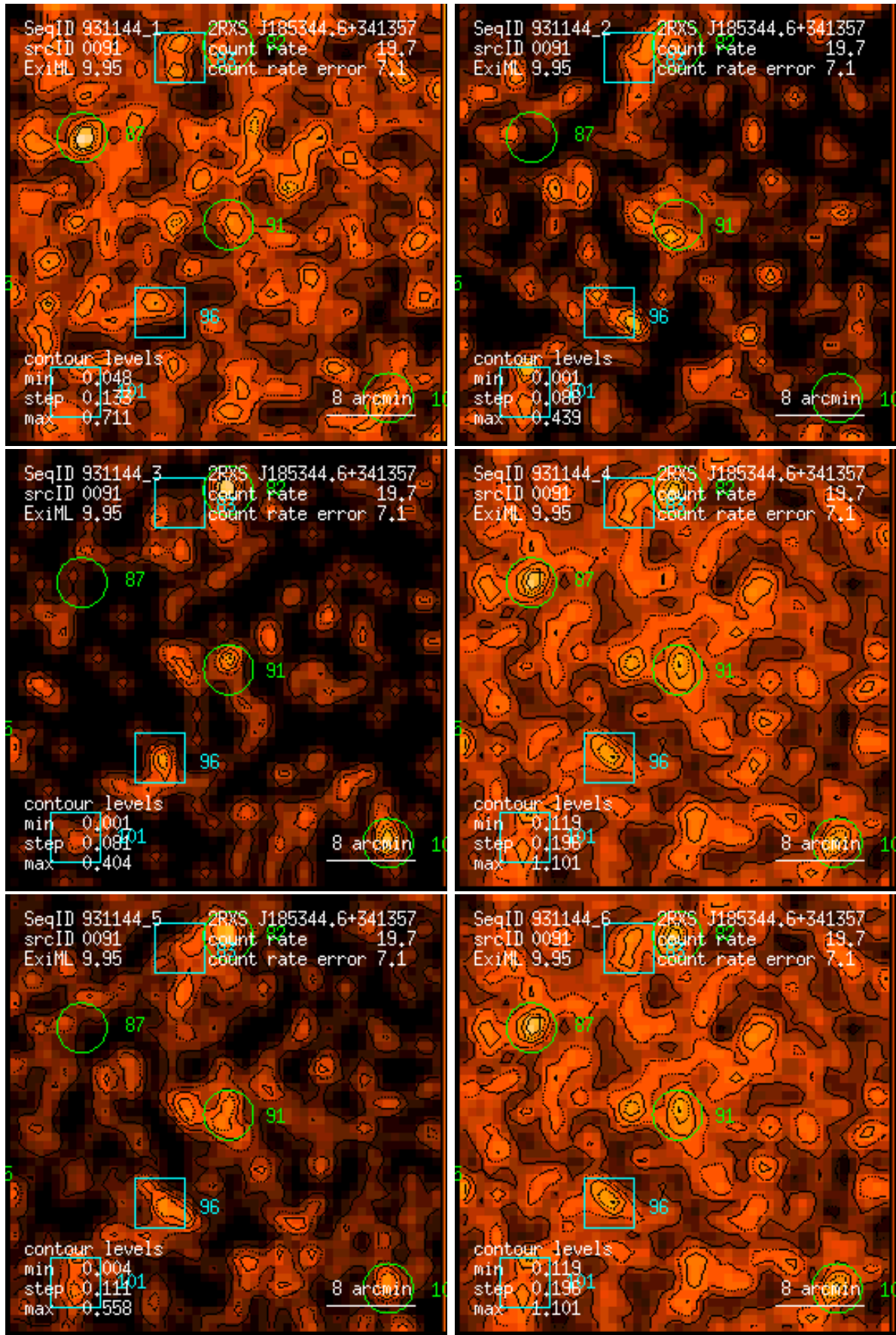
Figure 91: RASS 931144: detection 0091: band rate images, Gaussian filter: (1) PSPC channels 11 – 41, (2) 52 – 90, (3) 91 – 201, (4) 11 – 235, (5) 52 – 201, (6) 11 – 201. Broad band rates in counts/ks. Band rate contour levels in counts/ks/arcmin 2 .
