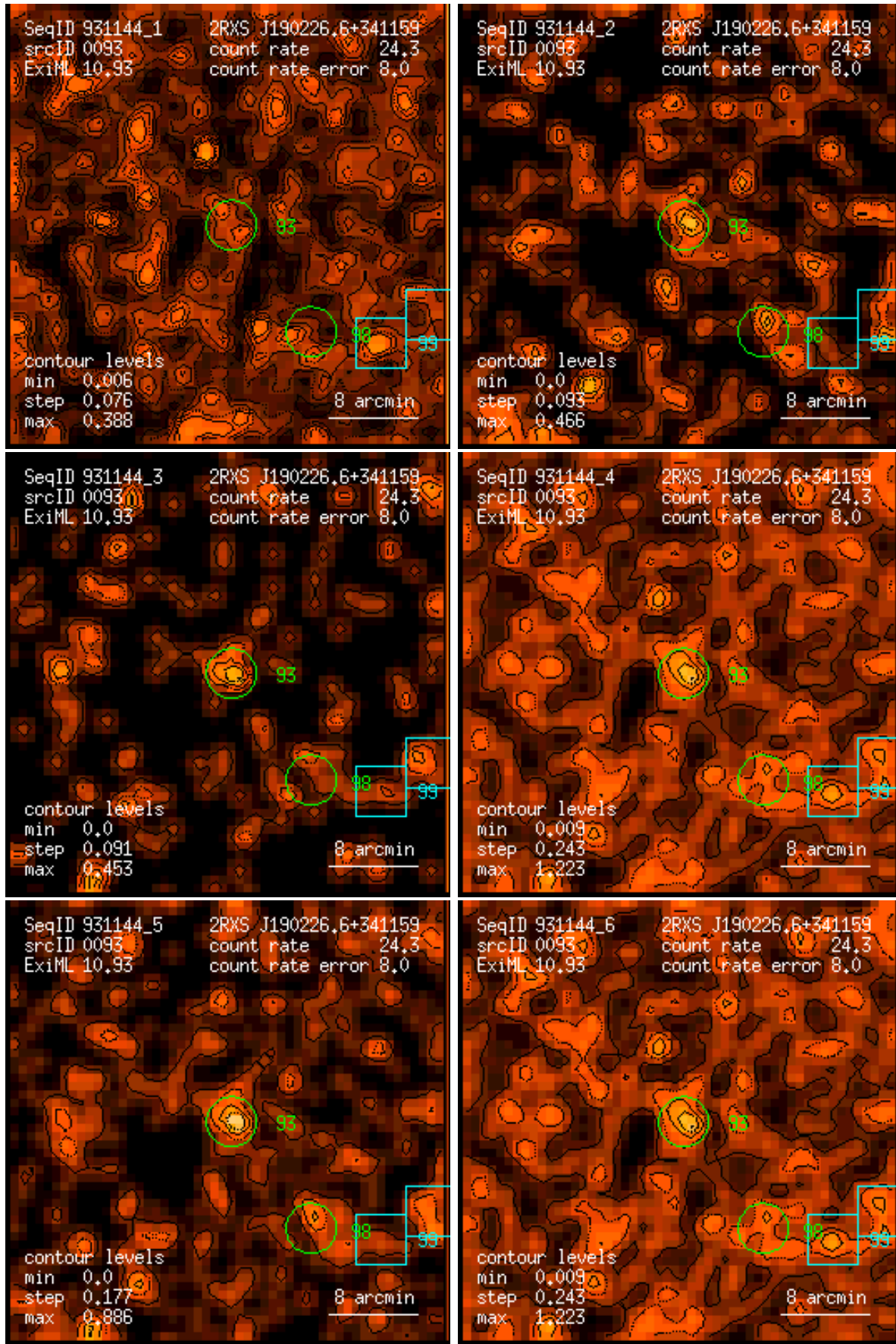
Figure 93: RASS 931144: detection 0093: band rate images, Gaussian filter: (1) PSPC channels 11 – 41, (2) 52 – 90, (3) 91 – 201, (4) 11 – 235, (5) 52 – 201, (6) 11 – 201. Broad band rates in counts/ks. Band rate contour levels in counts/ks/arcmin 2 .
