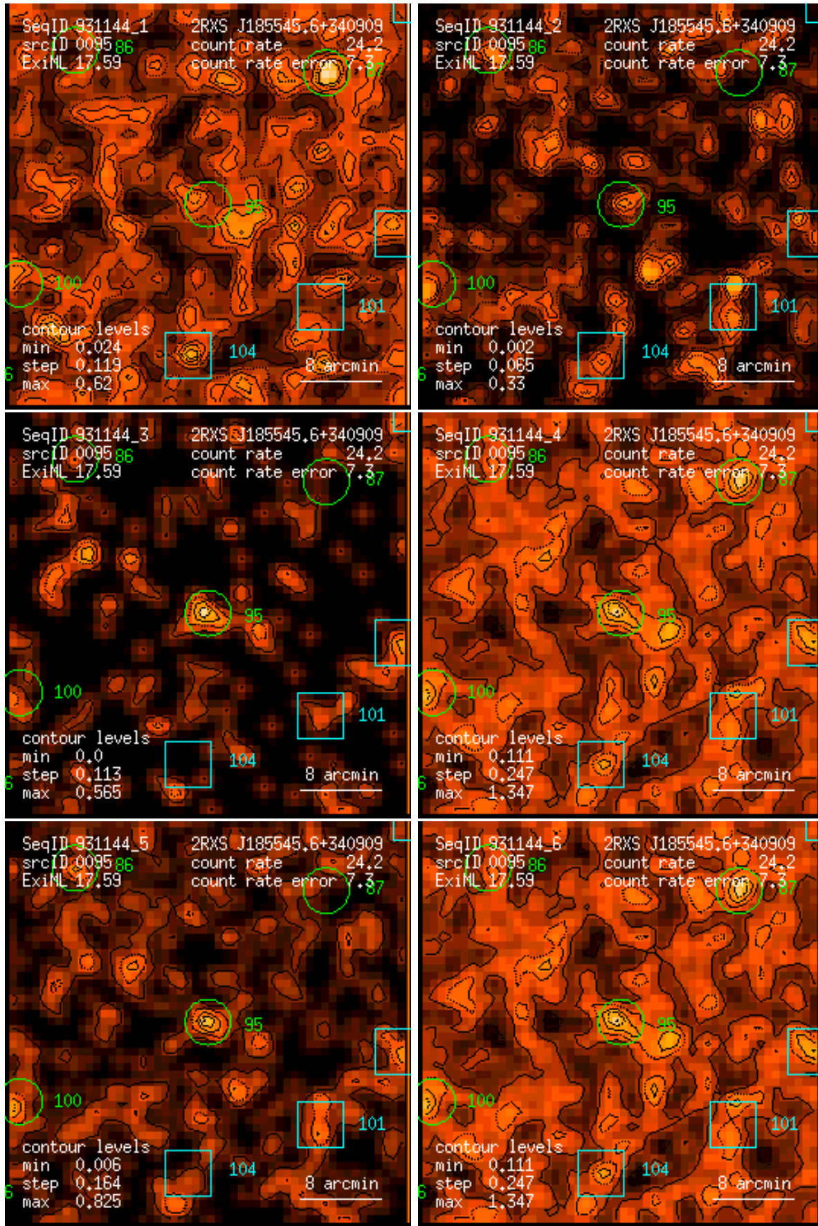
Figure 95: RASS 931144: detection 0095: band rate images, Gaussian filter: (1) PSPC channels 11 – 41, (2) 52 – 90, (3) 91 – 201, (4) 11 – 235, (5) 52 – 201, (6) 11 – 201. Broad band rates in counts/ks. Band rate contour levels in counts/ks/arcmin 2 .
