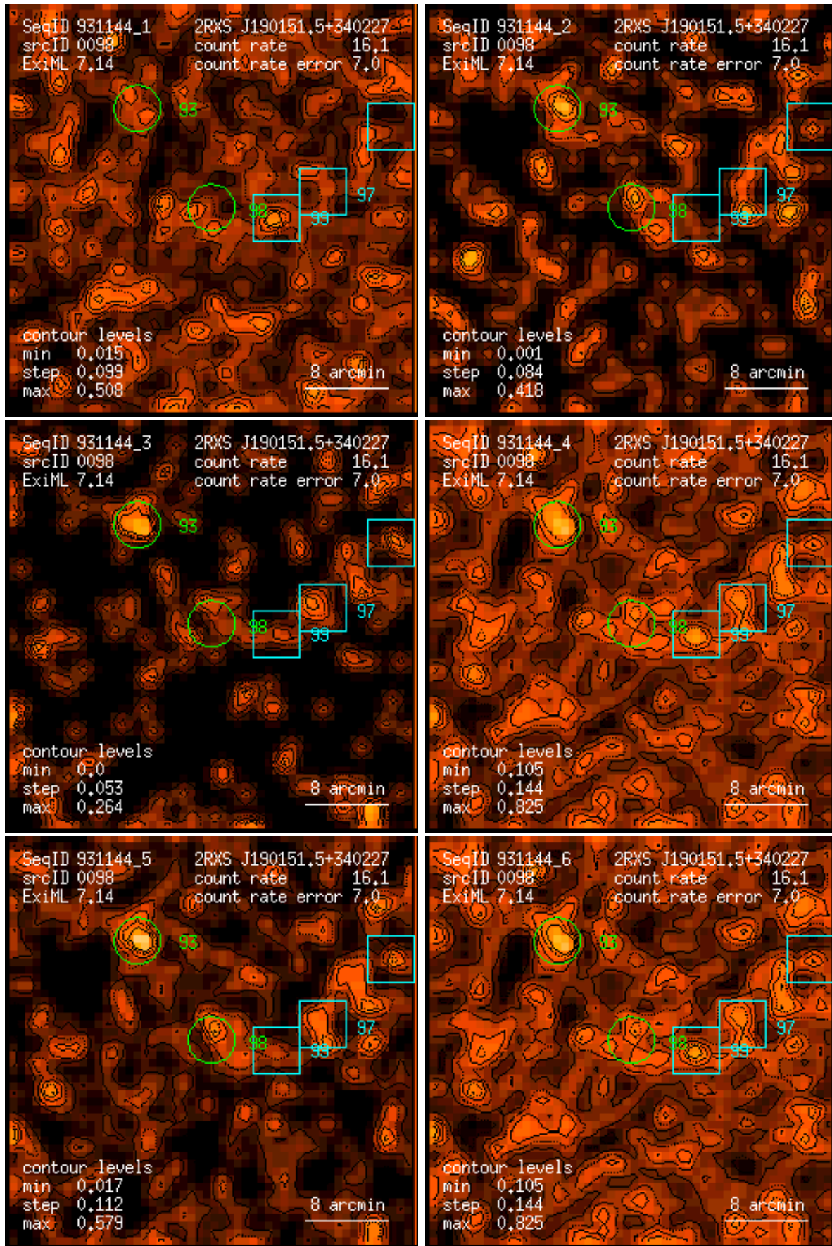
Figure 98: RASS 931144: detection 0098: band rate images, Gaussian filter: (1) PSPC channels 11 – 41, (2) 52 – 90, (3) 91 – 201, (4) 11 – 235, (5) 52 – 201, (6) 11 – 201. Broad band rates in counts/ks. Band rate contour levels in counts/ks/arcmin 2 .
