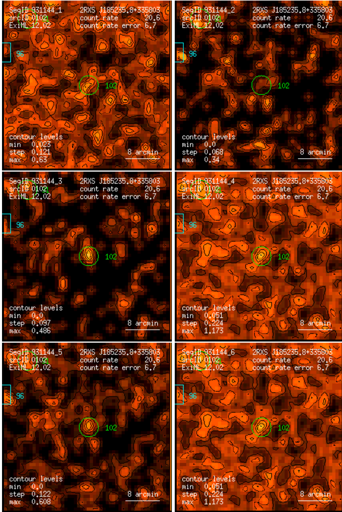
Figure 102: RASS 931144: detection 0102: band rate images, Gaussian filter: (1) PSPC channels 11 – 41, (2) 52 – 90, (3) 91 – 201, (4) 11 – 235, (5) 52 – 201, (6) 11 – 201. Broad band rates in counts/ks. Band rate contour levels in counts/ks/arcmin 2 .
