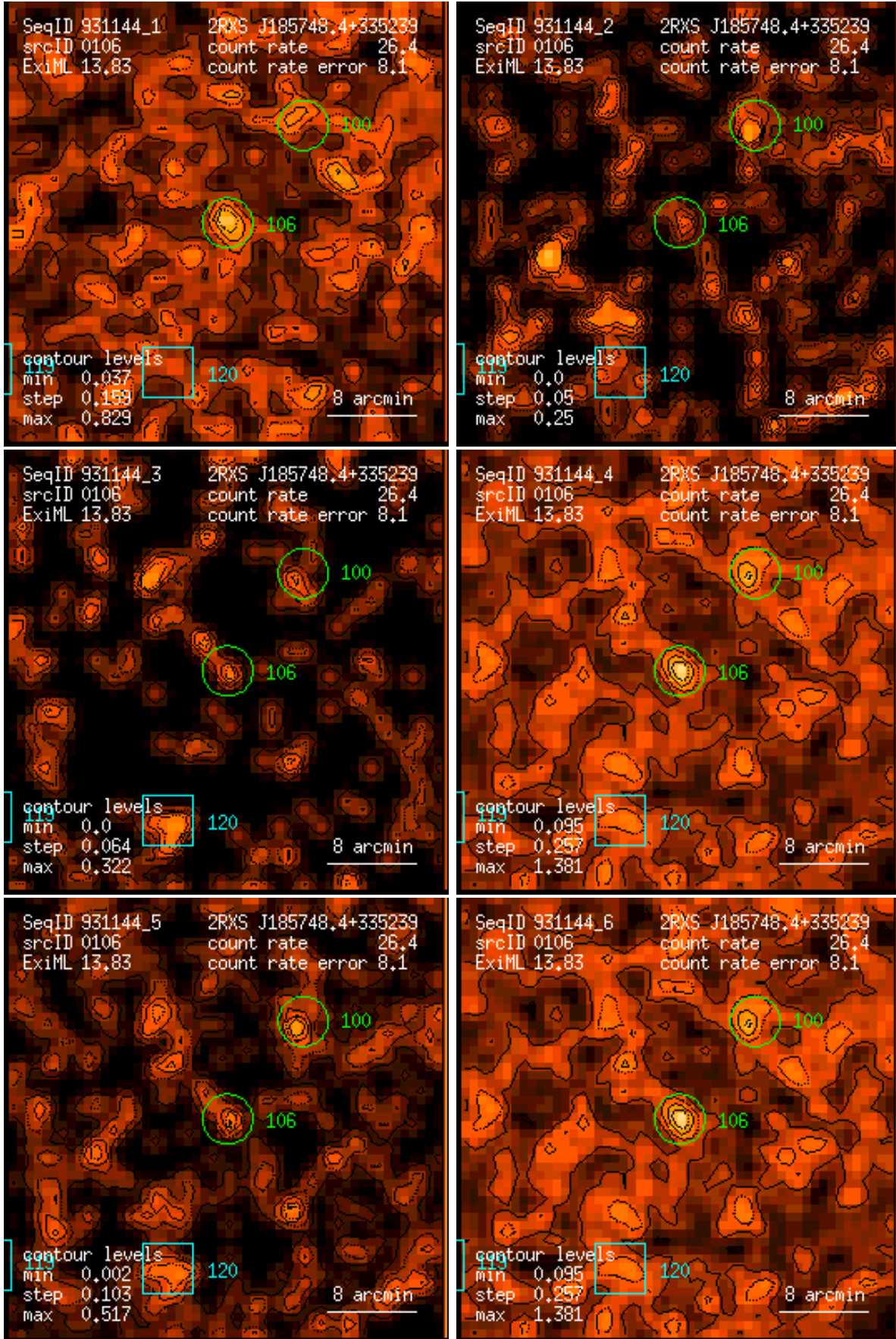
Figure 106: RASS 931144: detection 0106: band rate images, Gaussian filter: (1) PSPC channels 11 – 41, (2) 52 – 90, (3) 91 – 201, (4) 11 – 235, (5) 52 – 201, (6) 11 – 201. Broad band rates in counts/ks. Band rate contour levels in counts/ks/arcmin 2 .
