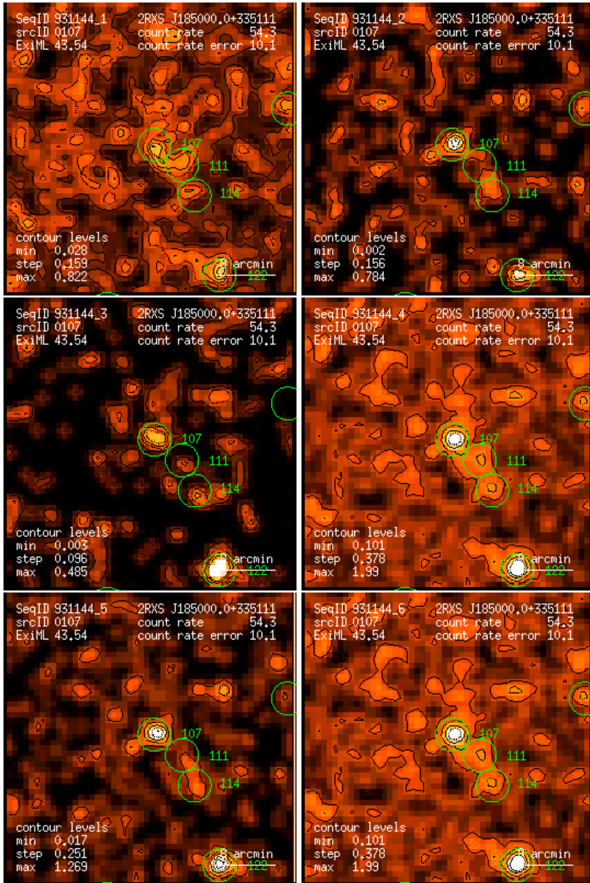
Figure 107: RASS 931144: detection 0107: band rate images, Gaussian filter: (1) PSPC channels 11 – 41, (2) 52 – 90, (3) 91 – 201, (4) 11 – 235, (5) 52 – 201, (6) 11 – 201. Broad band rates in counts/ks. Band rate contour levels in counts/ks/arcmin 2 .
