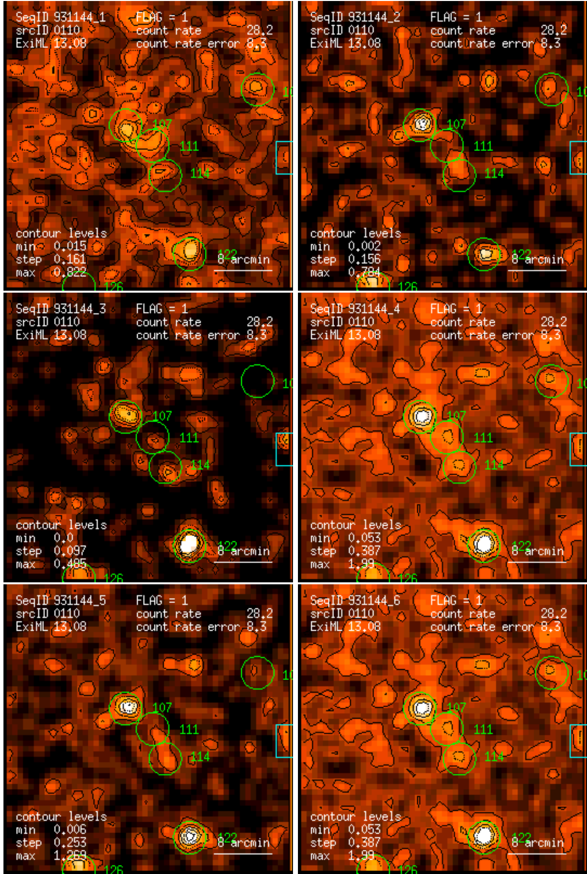
Figure 110: RASS 931144: detection 0110: band rate images, Gaussian filter: (1) PSPC channels 11 – 41, (2) 52 – 90, (3) 91 – 201, (4) 11 – 235, (5) 52 – 201, (6) 11 – 201. Broad band rates in counts/ks. Band rate contour levels in counts/ks/arcmin 2 .
