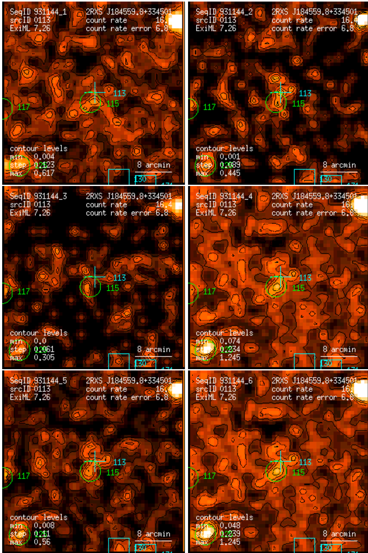
Figure 113: RASS 931144: detection 0113: band rate images, Gaussian filter: (1) PSPC channels 11 – 41, (2) 52 – 90, (3) 91 – 201, (4) 11 – 235, (5) 52 – 201, (6) 11 – 201. Broad band rates in counts/ks. Band rate contour levels in counts/ks/arcmin 2 .
