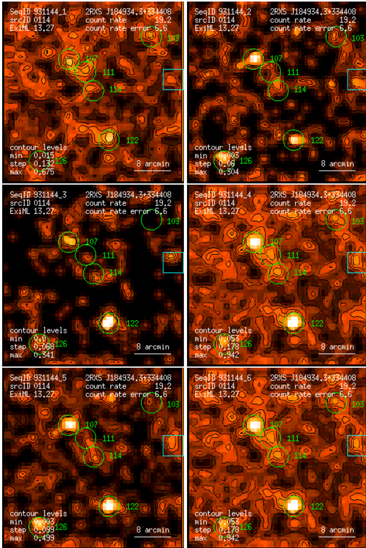
Figure 114: RASS 931144: detection 0114: band rate images, Gaussian filter: (1) PSPC channels 11 – 41, (2) 52 – 90, (3) 91 – 201, (4) 11 – 235, (5) 52 – 201, (6) 11 – 201. Broad band rates in counts/ks. Band rate contour levels in counts/ks/arcmin 2 .
