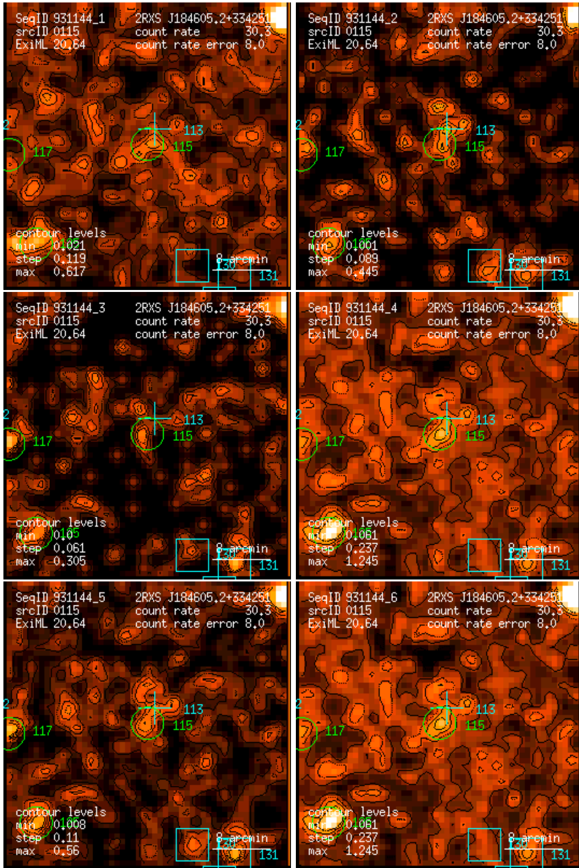
Figure 115: RASS 931144: detection 0115: band rate images, Gaussian filter: (1) PSPC channels 11 – 41, (2) 52 – 90, (3) 91 – 201, (4) 11 – 235, (5) 52 – 201, (6) 11 – 201. Broad band rates in counts/ks. Band rate contour levels in counts/ks/arcmin 2 .
