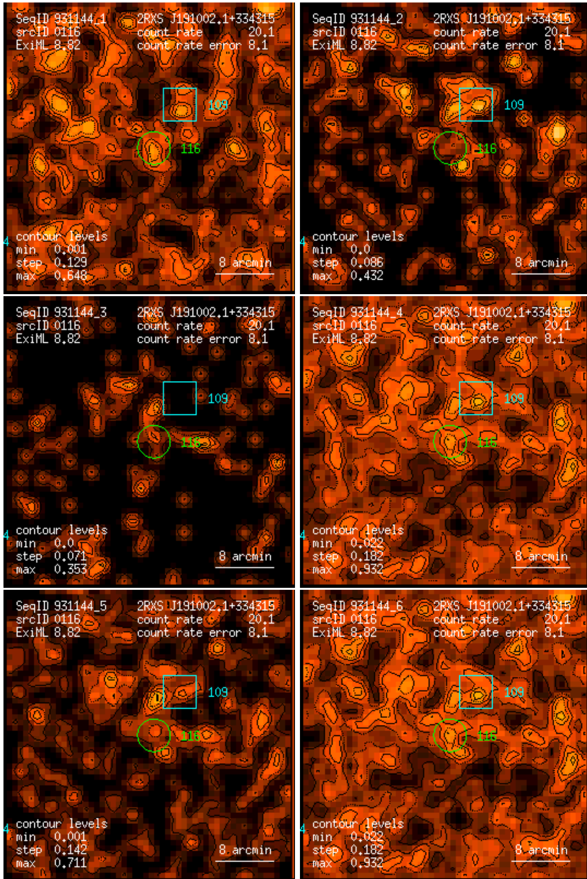
Figure 116: RASS 931144: detection 0116: band rate images, Gaussian filter: (1) PSPC channels 11 – 41, (2) 52 – 90, (3) 91 – 201, (4) 11 – 235, (5) 52 – 201, (6) 11 – 201. Broad band rates in counts/ks. Band rate contour levels in counts/ks/arcmin 2 .
