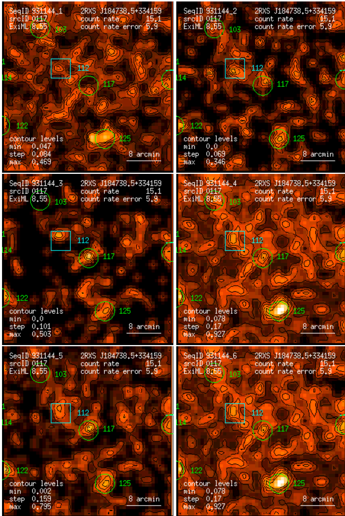
Figure 117: RASS 931144: detection 0117: band rate images, Gaussian filter: (1) PSPC channels 11 – 41, (2) 52 – 90, (3) 91 – 201, (4) 11 – 235, (5) 52 – 201, (6) 11 – 201. Broad band rates in counts/ks. Band rate contour levels in counts/ks/arcmin 2 .
