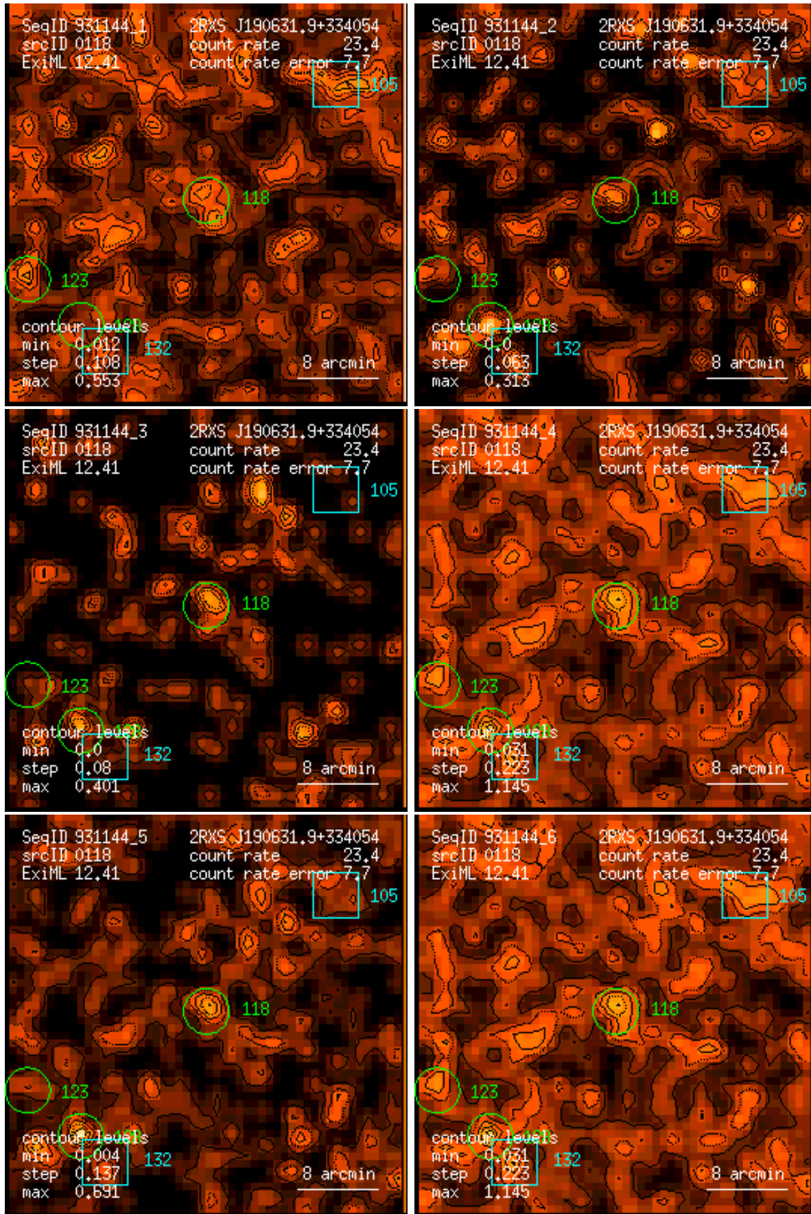
Figure 118: RASS 931144: detection 0118: band rate images, Gaussian filter: (1) PSPC channels 11 – 41, (2) 52 – 90, (3) 91 – 201, (4) 11 – 235, (5) 52 – 201, (6) 11 – 201. Broad band rates in counts/ks. Band rate contour levels in counts/ks/arcmin 2 .
