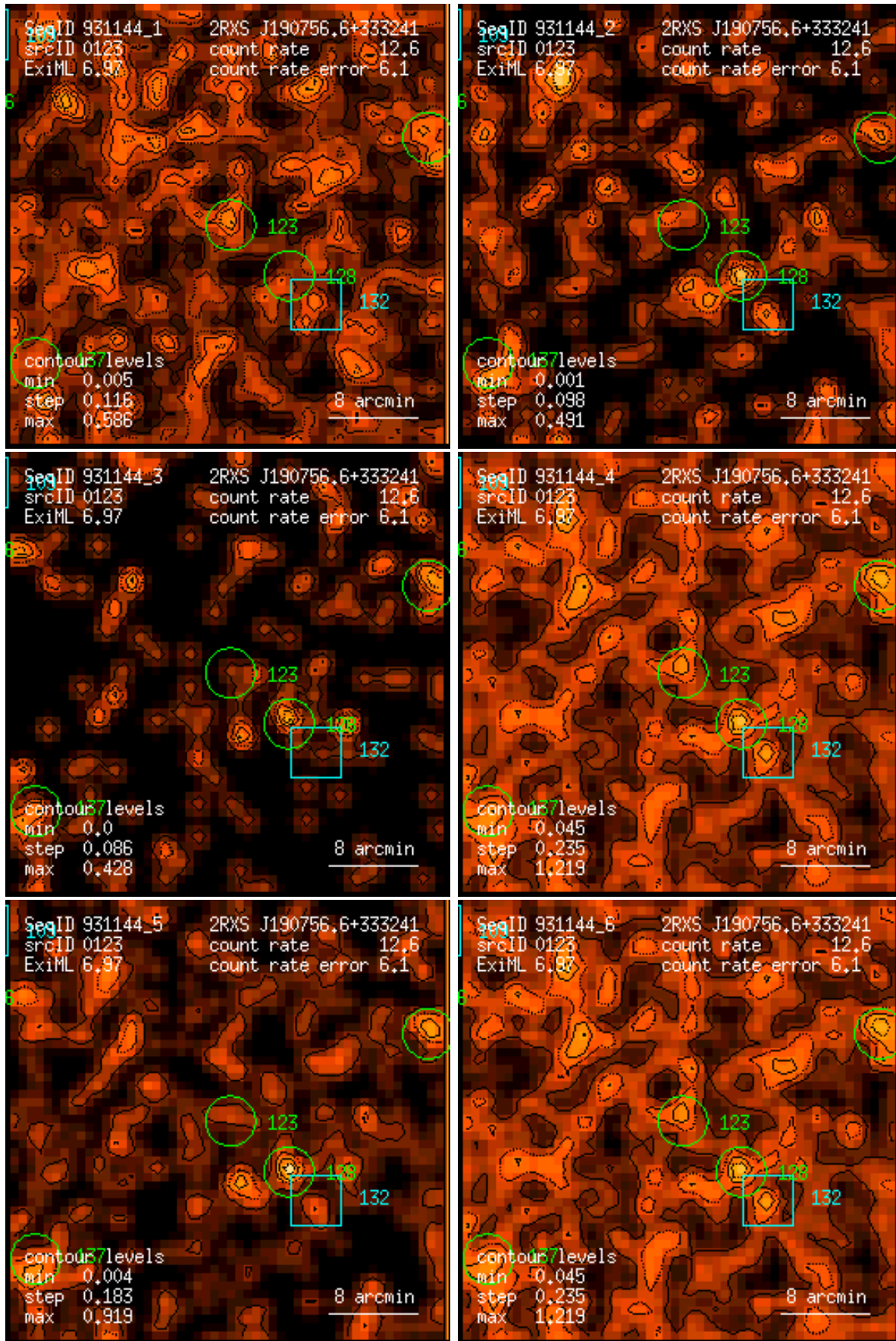
Figure 123: RASS 931144: detection 0123: band rate images, Gaussian filter: (1) PSPC channels 11 – 41, (2) 52 – 90, (3) 91 – 201, (4) 11 – 235, (5) 52 – 201, (6) 11 – 201. Broad band rates in counts/ks. Band rate contour levels in counts/ks/arcmin 2 .
