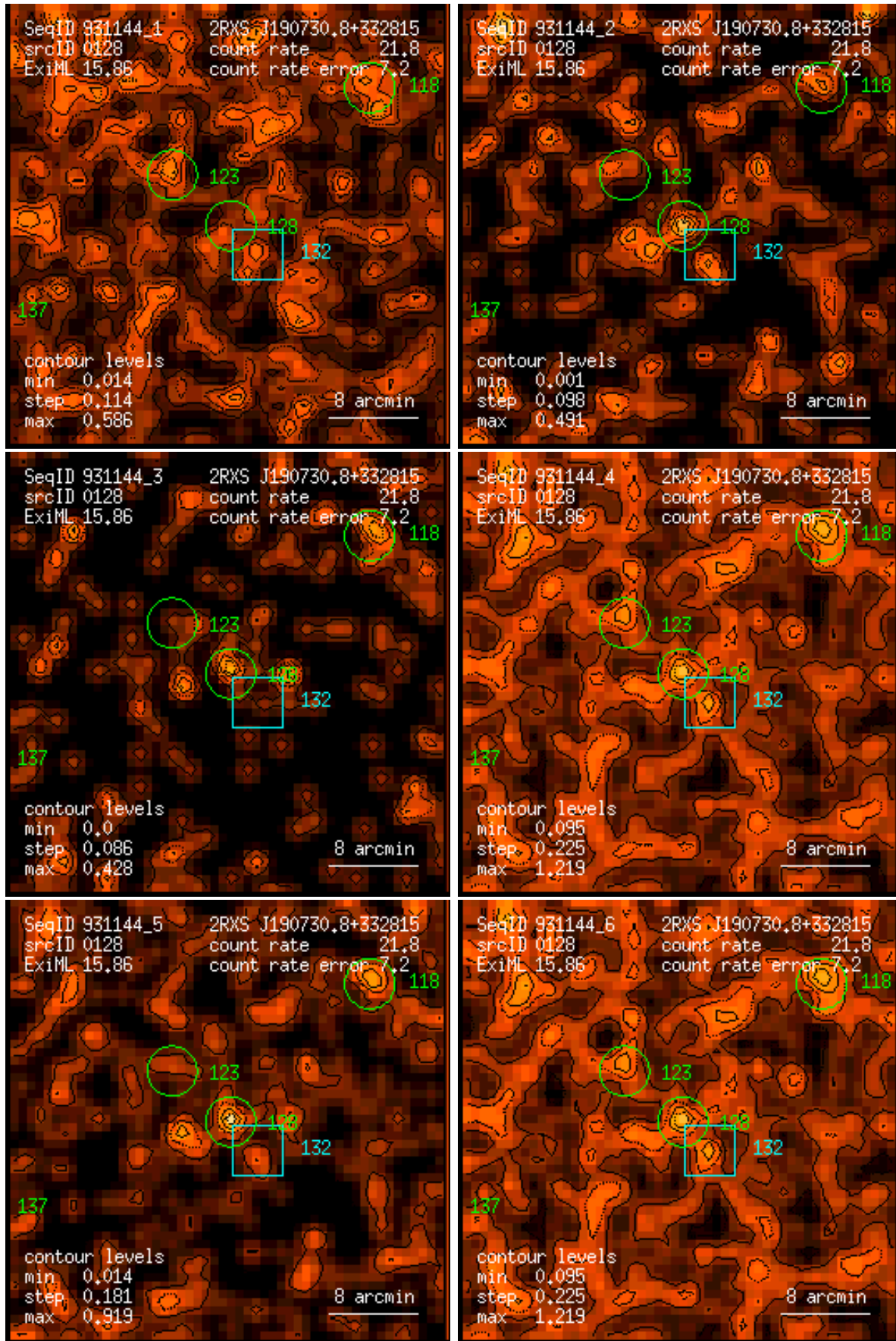
Figure 128: RASS 931144: detection 0128: band rate images, Gaussian filter: (1) PSPC channels 11 – 41, (2) 52 – 90, (3) 91 – 201, (4) 11 – 235, (5) 52 – 201, (6) 11 – 201. Broad band rates in counts/ks. Band rate contour levels in counts/ks/arcmin 2 .
