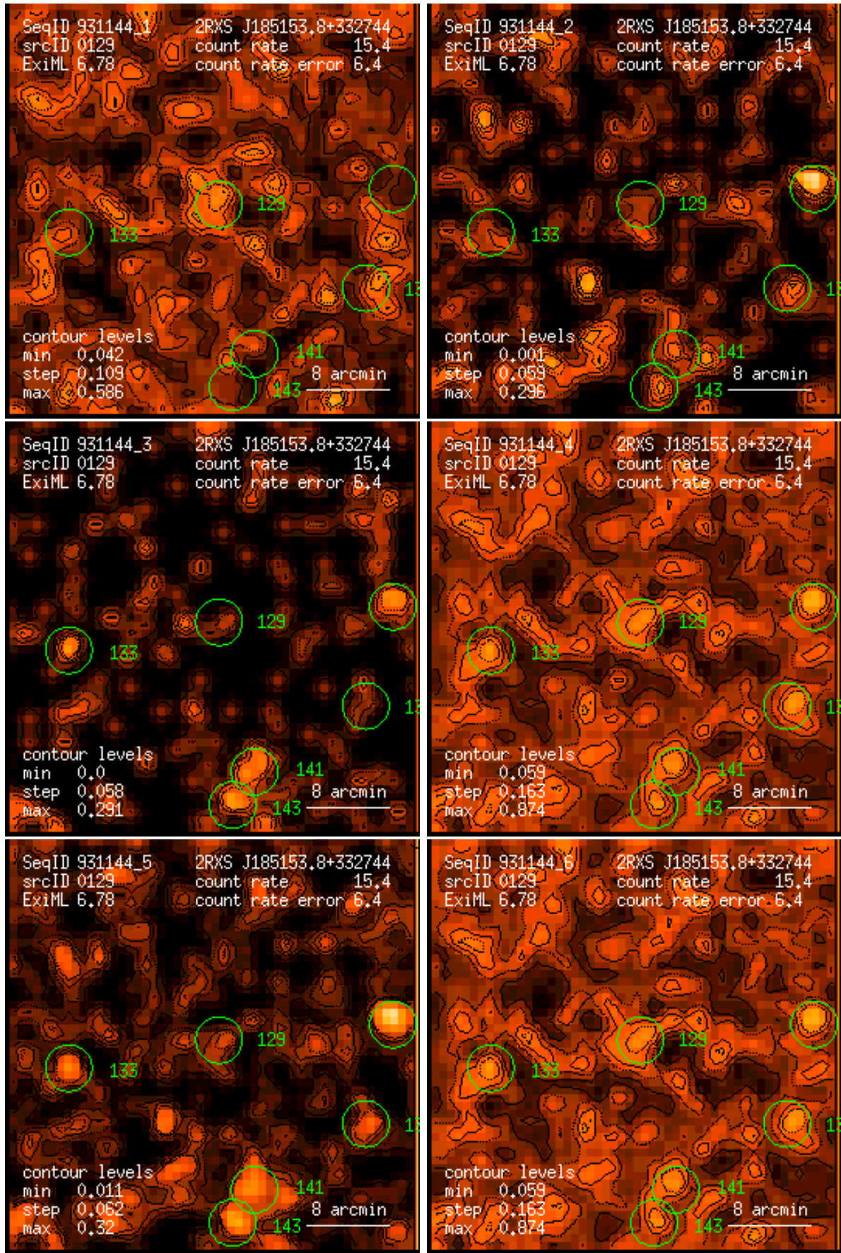
Figure 129: RASS 931144: detection 0129: band rate images, Gaussian filter: (1) PSPC channels 11 – 41, (2) 52 – 90, (3) 91 – 201, (4) 11 – 235, (5) 52 – 201, (6) 11 – 201. Broad band rates in counts/ks. Band rate contour levels in counts/ks/arcmin 2 .
