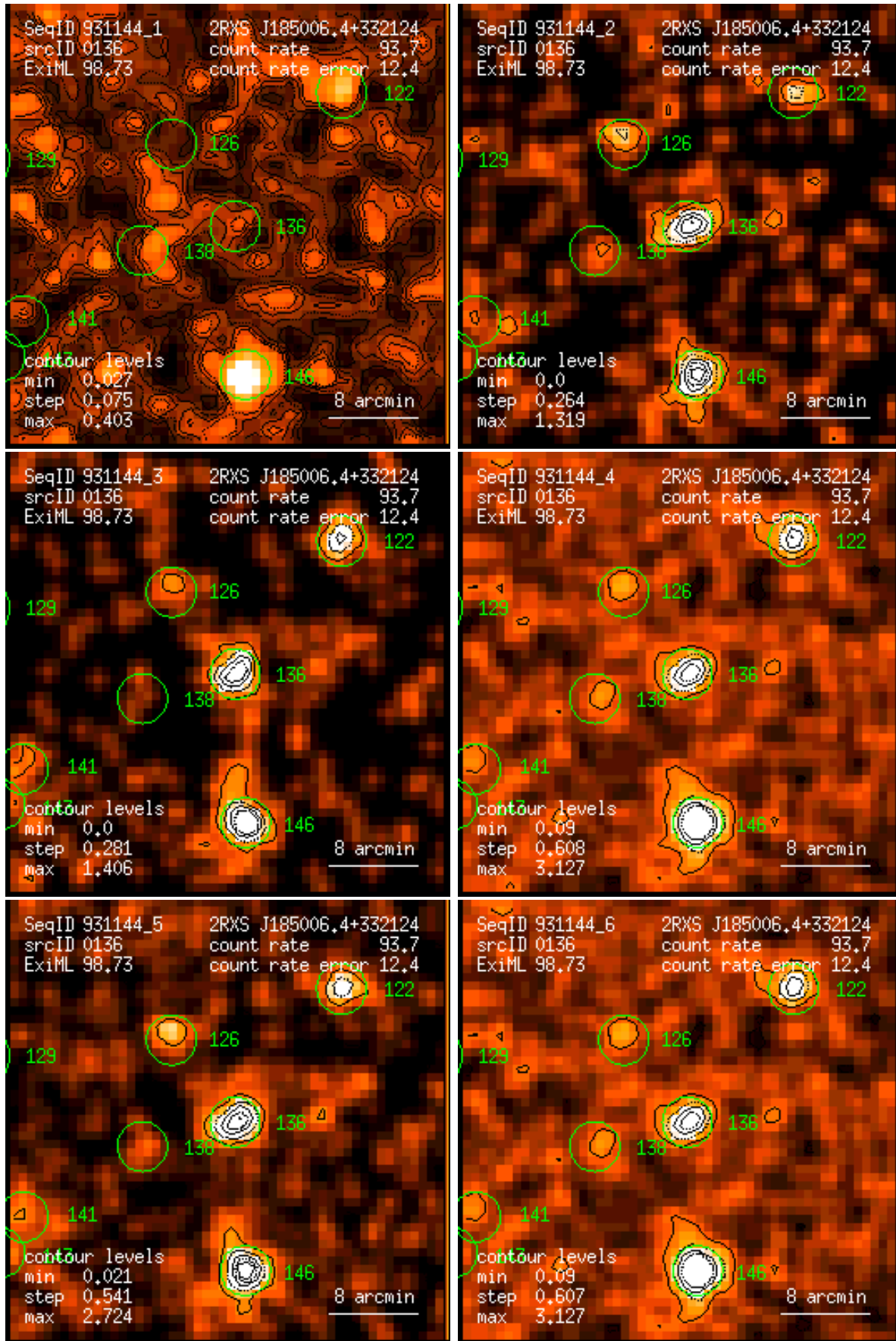
Figure 136: RASS 931144: detection 0136: band rate images, Gaussian filter: (1) PSPC channels 11 – 41, (2) 52 – 90, (3) 91 – 201, (4) 11 – 235, (5) 52 – 201, (6) 11 – 201. Broad band rates in counts/ks. Band rate contour levels in counts/ks/arcmin 2 .
