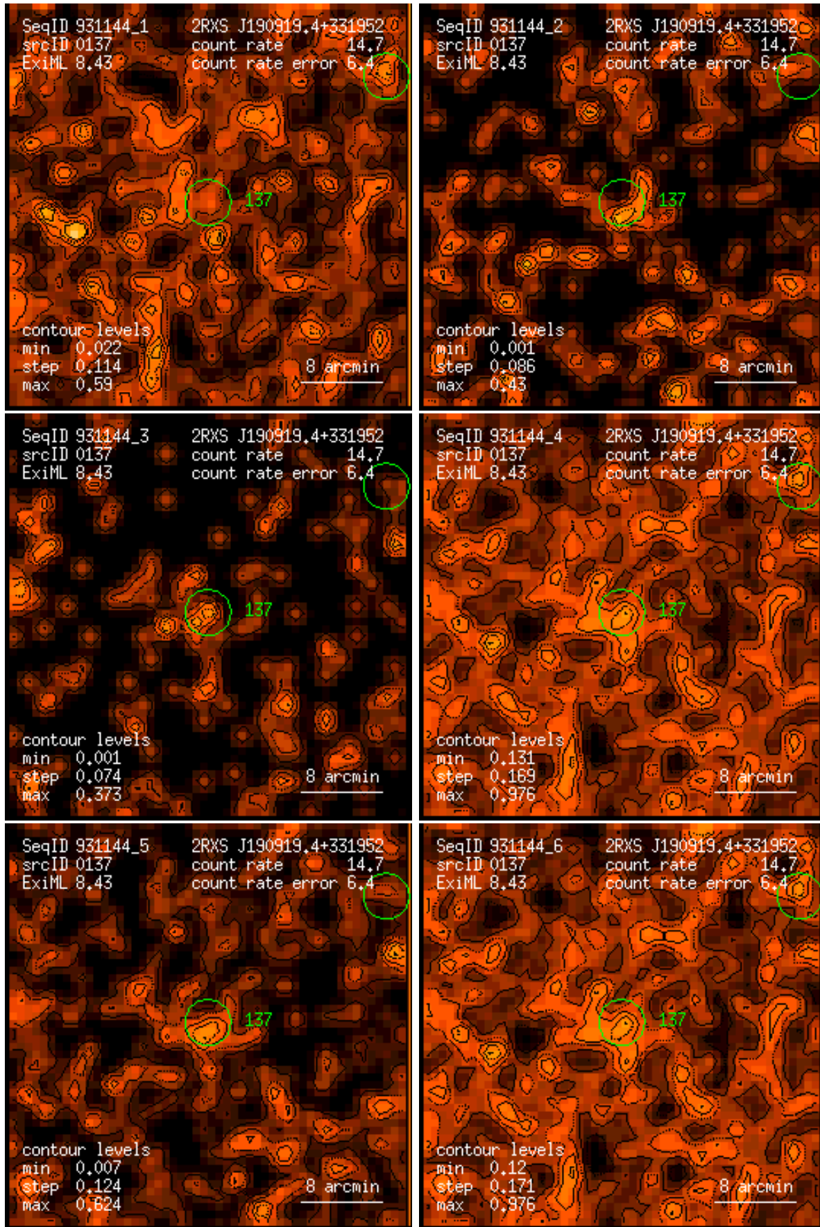
Figure 137: RASS 931144: detection 0137: band rate images, Gaussian filter: (1) PSPC channels 11 – 41, (2) 52 – 90, (3) 91 – 201, (4) 11 – 235, (5) 52 – 201, (6) 11 – 201. Broad band rates in counts/ks. Band rate contour levels in counts/ks/arcmin 2 .
