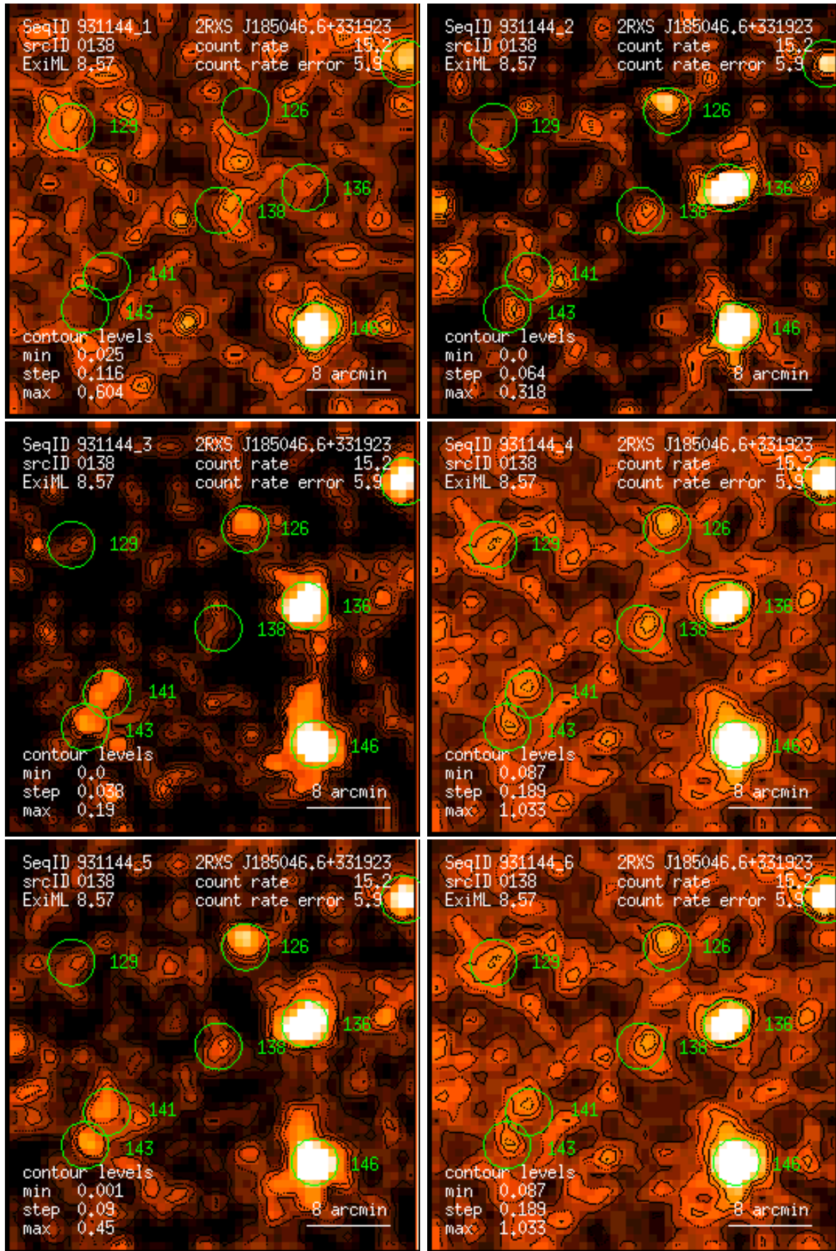
Figure 138: RASS 931144: detection 0138: band rate images, Gaussian filter: (1) PSPC channels 11 – 41, (2) 52 – 90, (3) 91 – 201, (4) 11 – 235, (5) 52 – 201, (6) 11 – 201. Broad band rates in counts/ks. Band rate contour levels in counts/ks/arcmin 2 .
