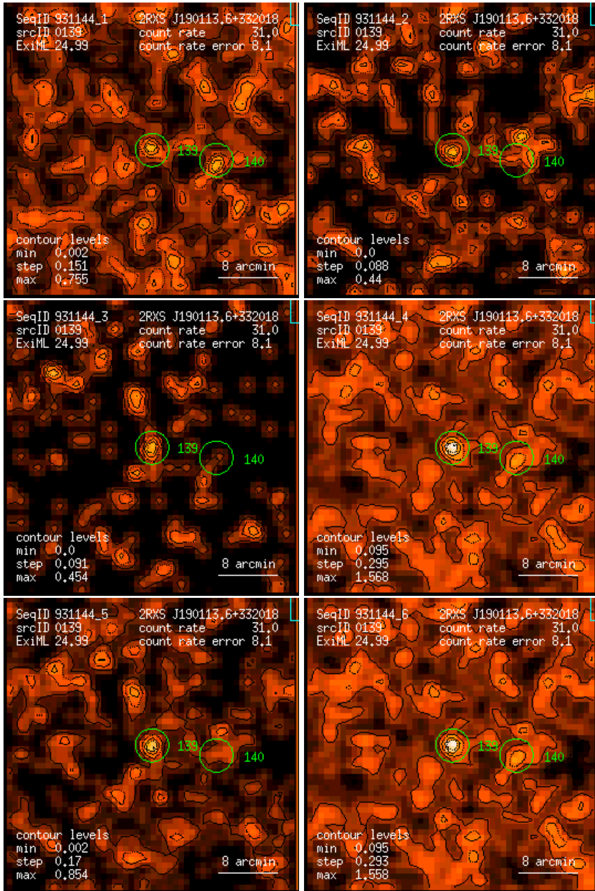
Figure 139: RASS 931144: detection 0139: band rate images, Gaussian filter: (1) PSPC channels 11 – 41, (2) 52 – 90, (3) 91 – 201, (4) 11 – 235, (5) 52 – 201, (6) 11 – 201. Broad band rates in counts/ks. Band rate contour levels in counts/ks/arcmin 2 .
