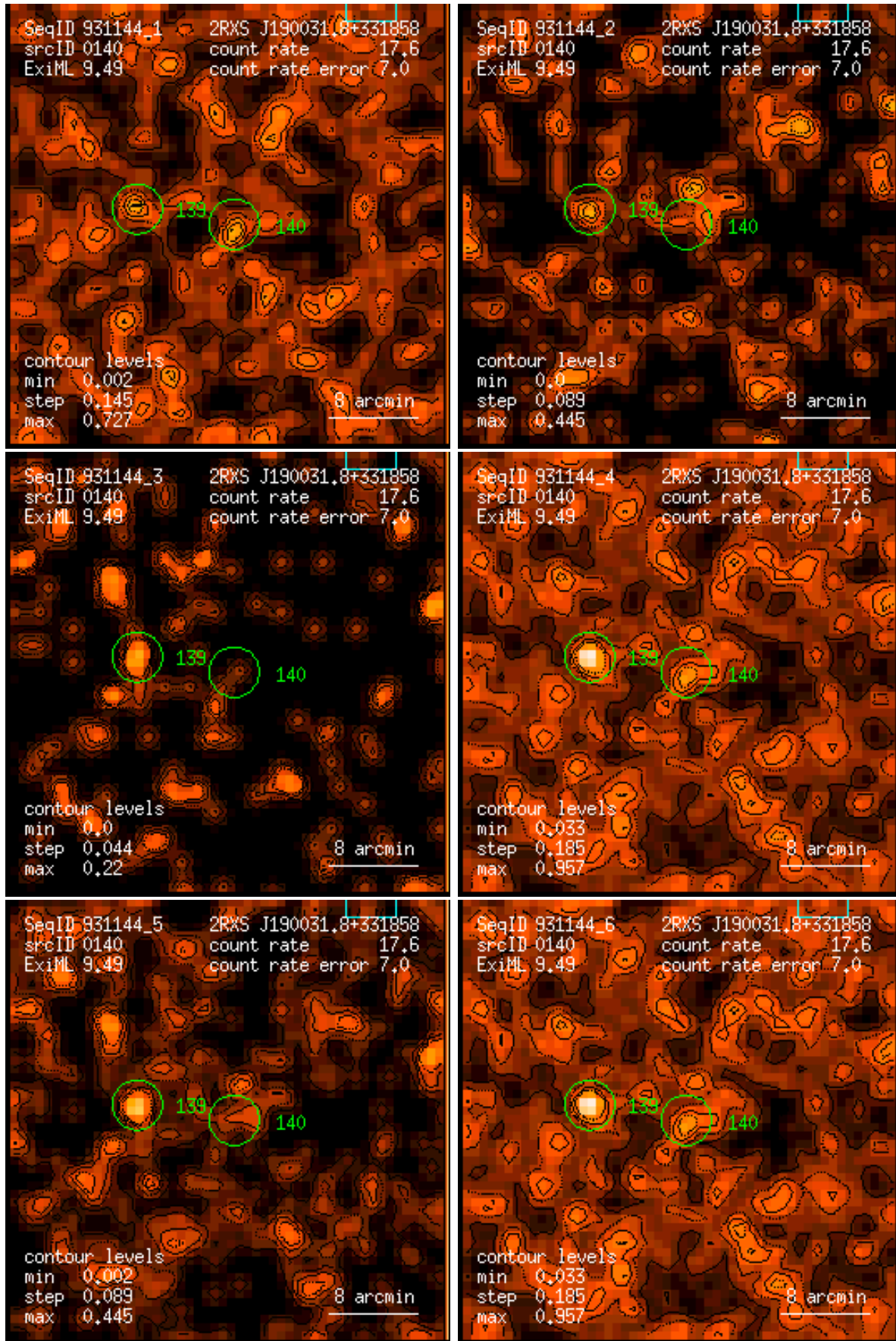
Figure 140: RASS 931144: detection 0140: band rate images, Gaussian filter: (1) PSPC channels 11 – 41, (2) 52 – 90, (3) 91 – 201, (4) 11 – 235, (5) 52 – 201, (6) 11 – 201. Broad band rates in counts/ks. Band rate contour levels in counts/ks/arcmin 2 .
