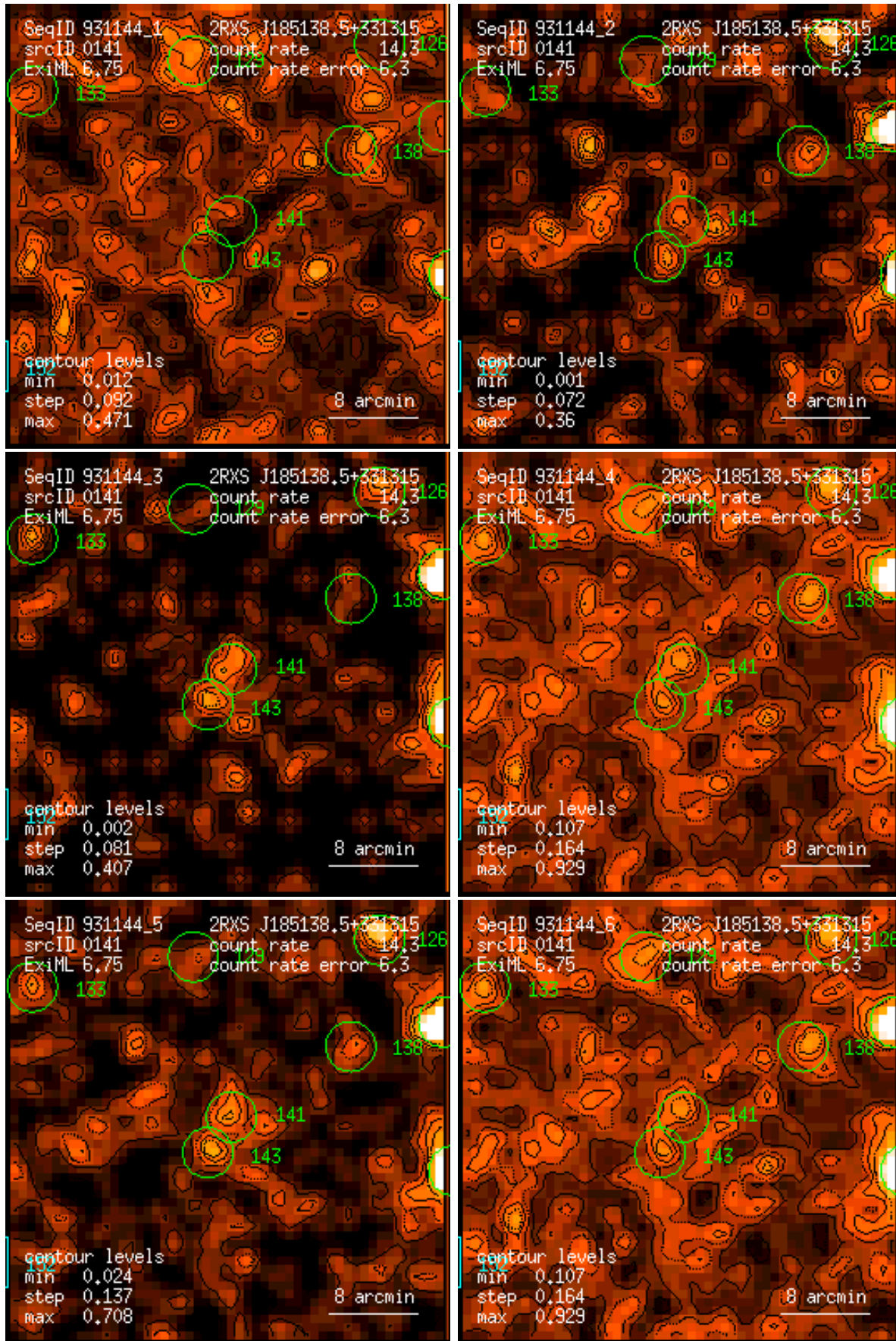
Figure 141: RASS 931144: detection 0141: band rate images, Gaussian filter: (1) PSPC channels 11 – 41, (2) 52 – 90, (3) 91 – 201, (4) 11 – 235, (5) 52 – 201, (6) 11 – 201. Broad band rates in counts/ks. Band rate contour levels in counts/ks/arcmin 2 .
