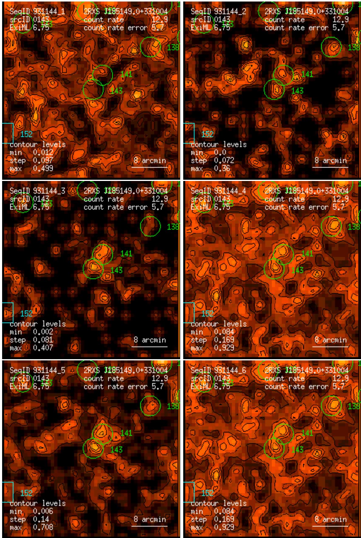
Figure 143: RASS 931144: detection 0143: band rate images, Gaussian filter: (1) PSPC channels 11 – 41, (2) 52 – 90, (3) 91 – 201, (4) 11 – 235, (5) 52 – 201, (6) 11 – 201. Broad band rates in counts/ks. Band rate contour levels in counts/ks/arcmin 2 .
