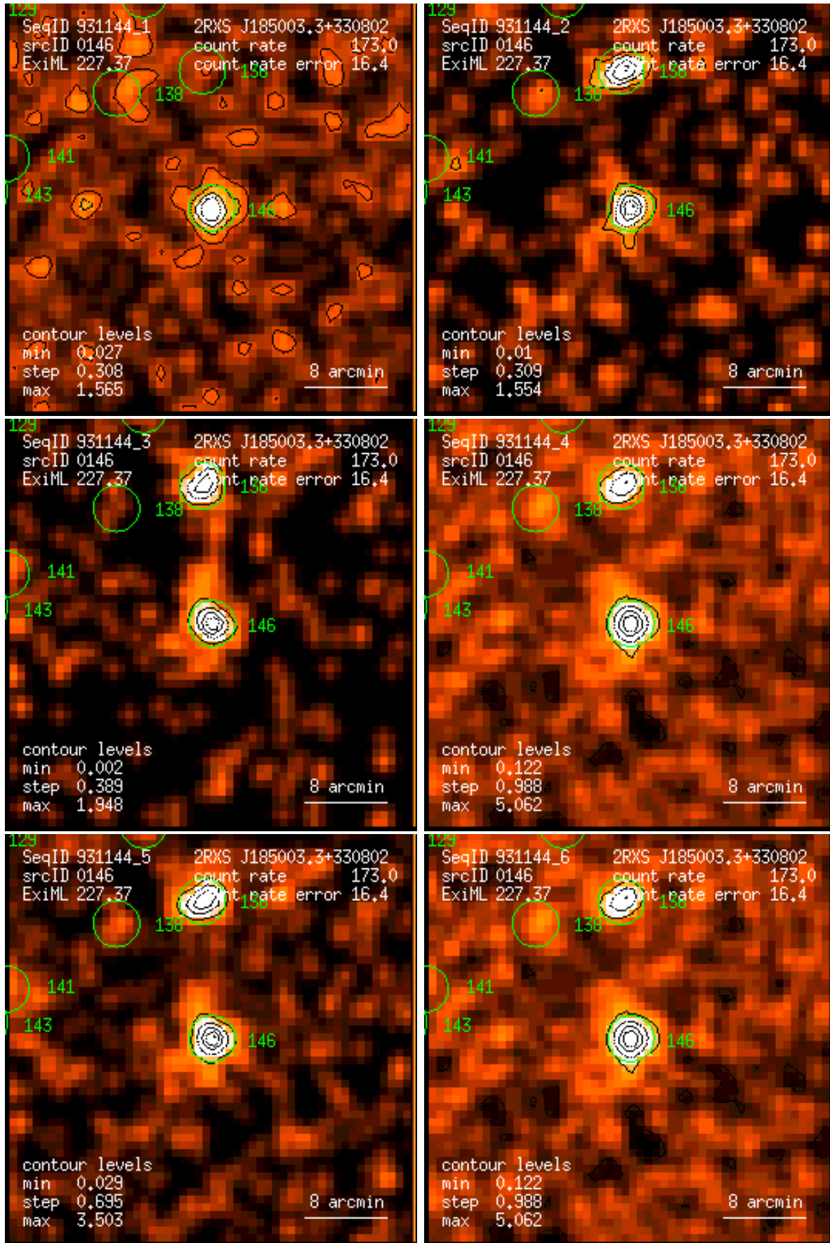
Figure 146: RASS 931144: detection 0146: band rate images, Gaussian filter: (1) PSPC channels 11 – 41, (2) 52 – 90, (3) 91 – 201, (4) 11 – 235, (5) 52 – 201, (6) 11 – 201. Broad band rates in counts/ks. Band rate contour levels in counts/ks/arcmin 2 .
