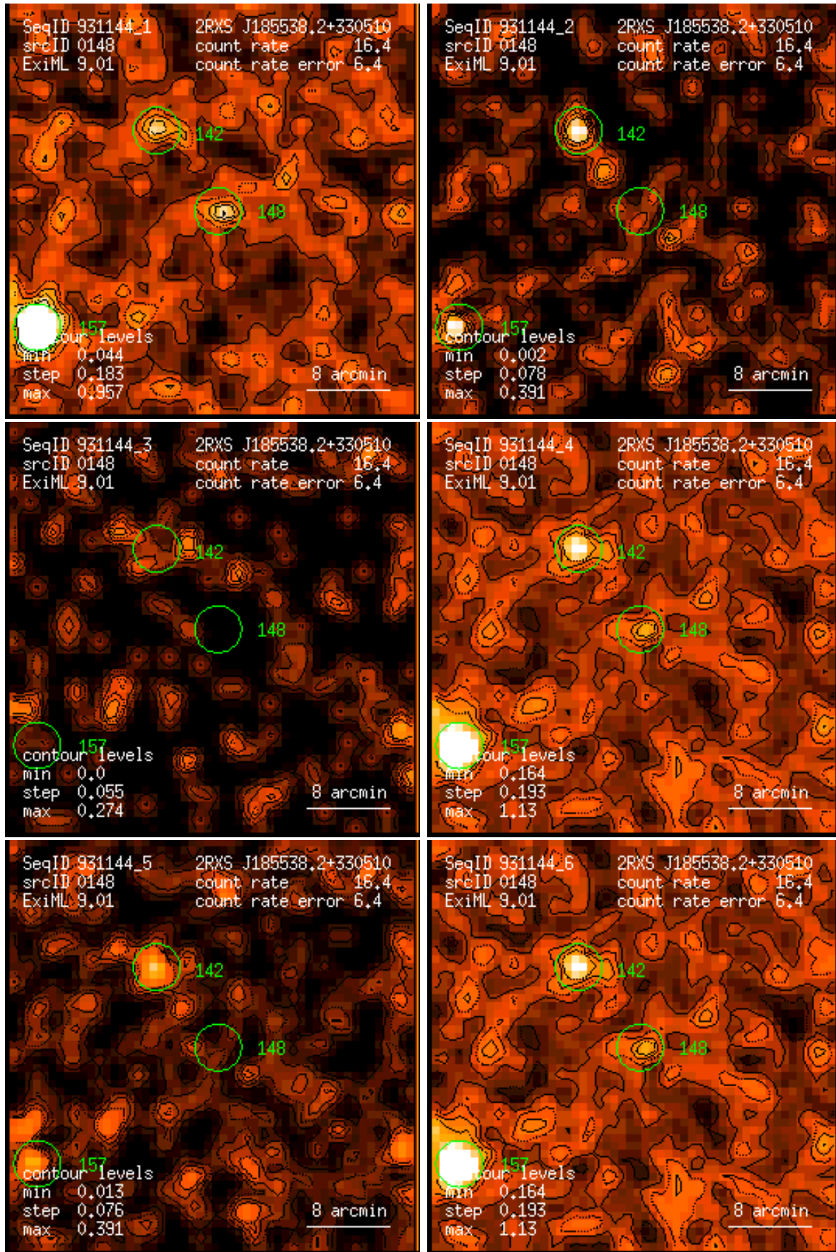
Figure 148: RASS 931144: detection 0148: band rate images, Gaussian filter: (1) PSPC channels 11 – 41, (2) 52 – 90, (3) 91 – 201, (4) 11 – 235, (5) 52 – 201, (6) 11 – 201. Broad band rates in counts/ks. Band rate contour levels in counts/ks/arcmin 2 .
