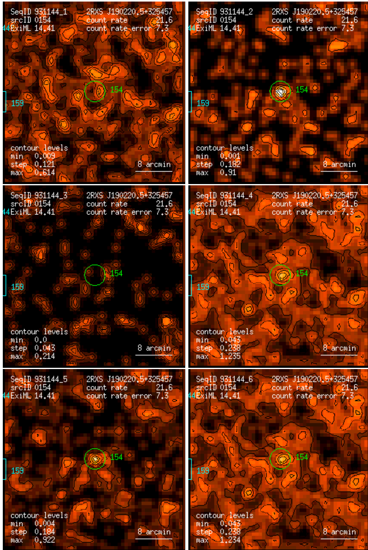
Figure 154: RASS 931144: detection 0154: band rate images, Gaussian filter: (1) PSPC channels 11 – 41, (2) 52 – 90, (3) 91 – 201, (4) 11 – 235, (5) 52 – 201, (6) 11 – 201. Broad band rates in counts/ks. Band rate contour levels in counts/ks/arcmin 2 .
