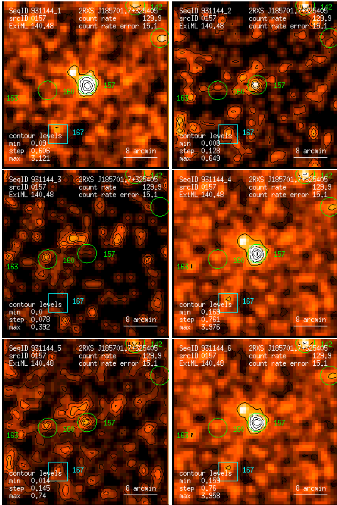
Figure 157: RASS 931144: detection 0157: band rate images, Gaussian filter: (1) PSPC channels 11 – 41, (2) 52 – 90, (3) 91 – 201, (4) 11 – 235, (5) 52 – 201, (6) 11 – 201. Broad band rates in counts/ks. Band rate contour levels in counts/ks/arcmin 2 .
