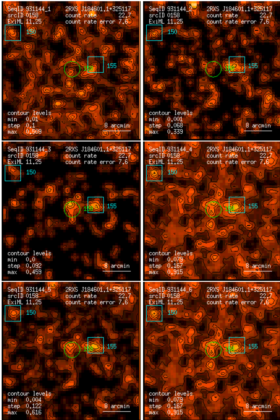
Figure 158: RASS 931144: detection 0158: band rate images, Gaussian filter: (1) PSPC channels 11 – 41, (2) 52 – 90, (3) 91 – 201, (4) 11 – 235, (5) 52 – 201, (6) 11 – 201. Broad band rates in counts/ks. Band rate contour levels in counts/ks/arcmin 2 .
