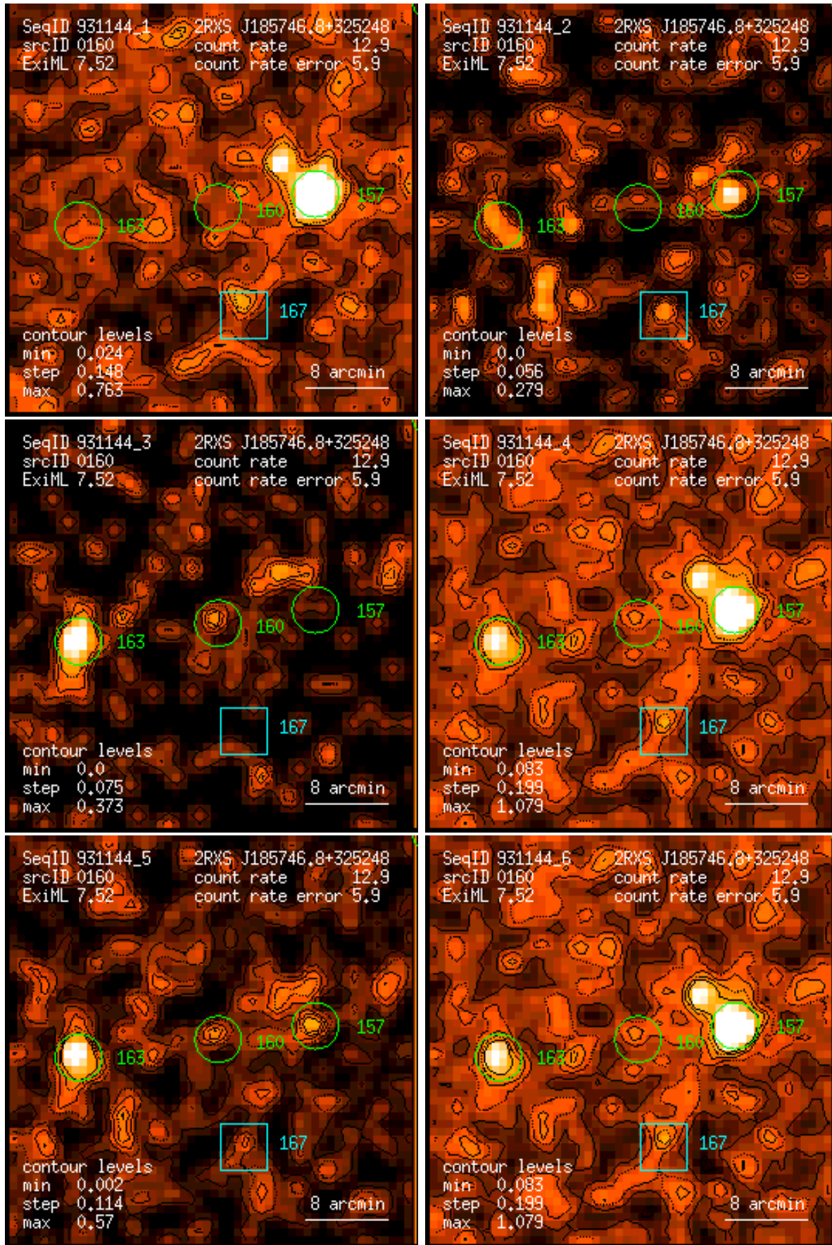
Figure 160: RASS 931144: detection 0160: band rate images, Gaussian filter: (1) PSPC channels 11 – 41, (2) 52 – 90, (3) 91 – 201, (4) 11 – 235, (5) 52 – 201, (6) 11 – 201. Broad band rates in counts/ks. Band rate contour levels in counts/ks/arcmin 2 .
