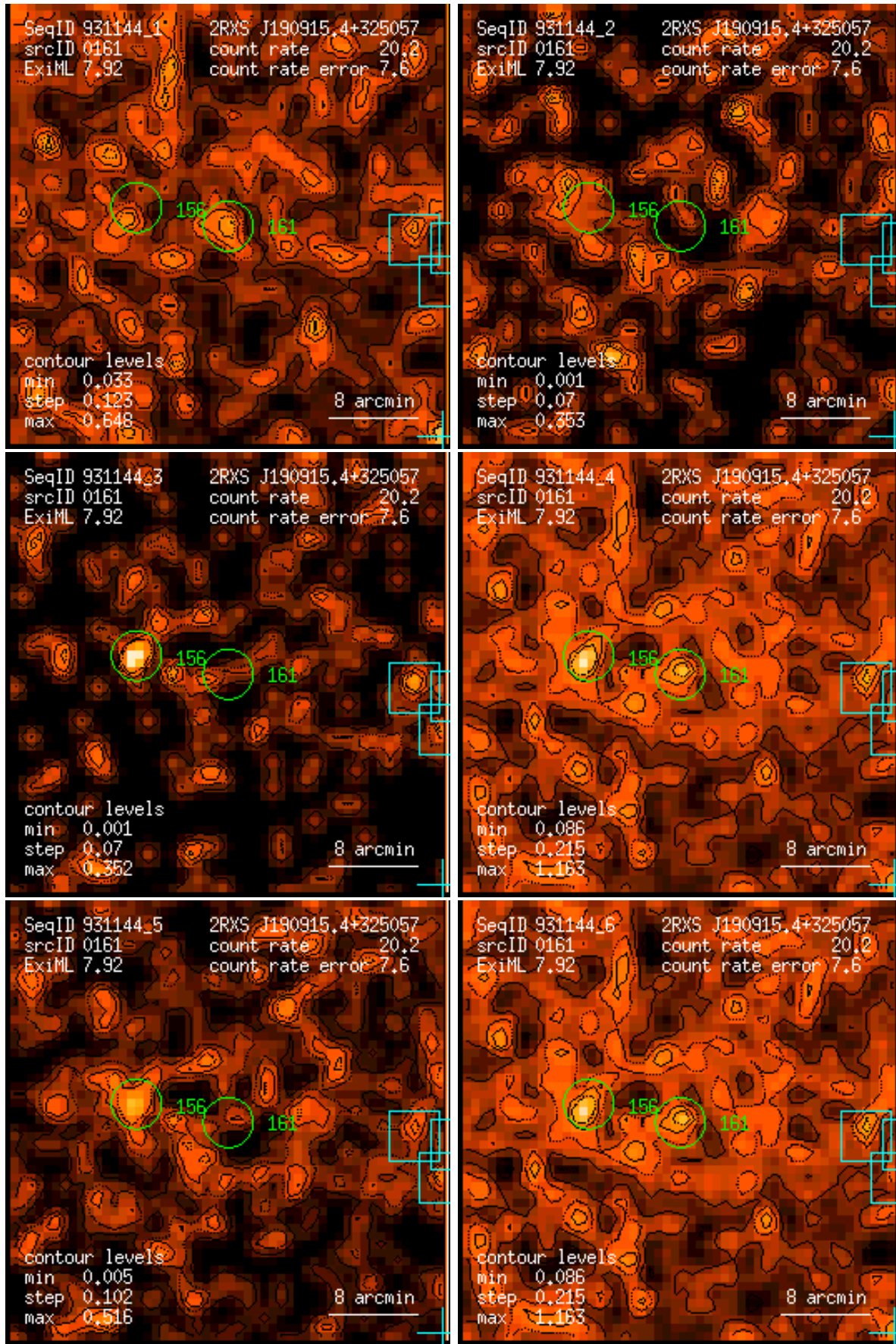
Figure 161: RASS 931144: detection 0161: band rate images, Gaussian filter: (1) PSPC channels 11 – 41, (2) 52 – 90, (3) 91 – 201, (4) 11 – 235, (5) 52 – 201, (6) 11 – 201. Broad band rates in counts/ks. Band rate contour levels in counts/ks/arcmin 2 .
