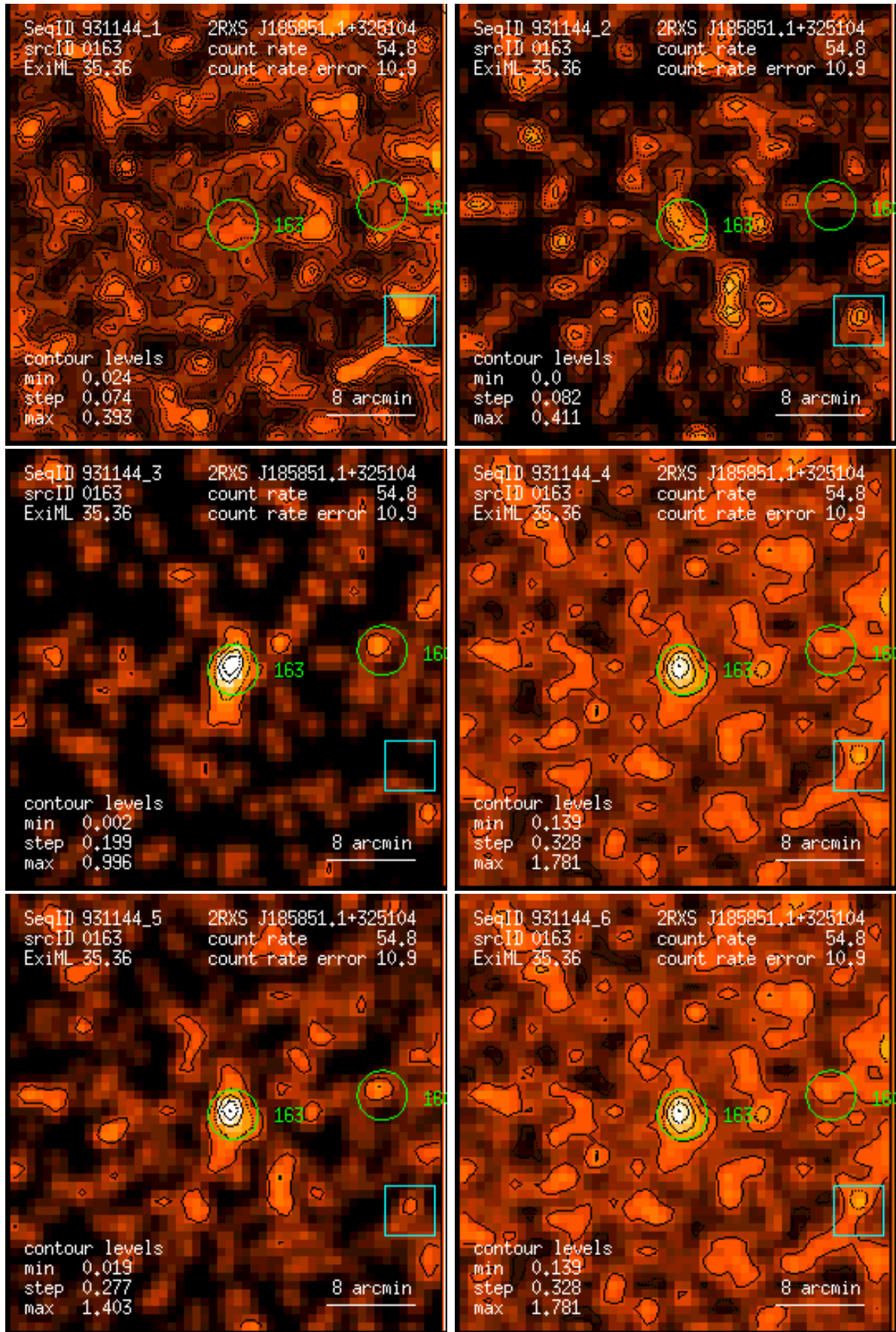
Figure 163: RASS 931144: detection 0163: band rate images, Gaussian filter: (1) PSPC channels 11 – 41, (2) 52 – 90, (3) 91 – 201, (4) 11 – 235, (5) 52 – 201, (6) 11 – 201. Broad band rates in counts/ks. Band rate contour levels in counts/ks/arcmin 2 .
