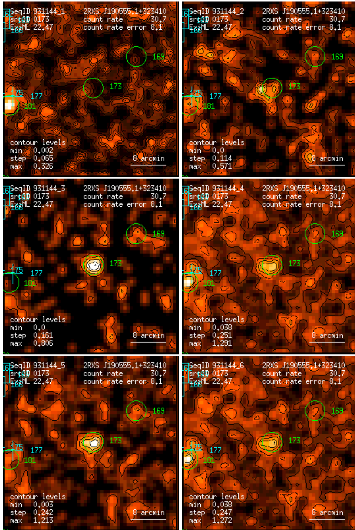
Figure 173: RASS 931144: detection 0173: band rate images, Gaussian filter: (1) PSPC channels 11 – 41, (2) 52 – 90, (3) 91 – 201, (4) 11 – 235, (5) 52 – 201, (6) 11 – 201. Broad band rates in counts/ks. Band rate contour levels in counts/ks/arcmin 2 .
