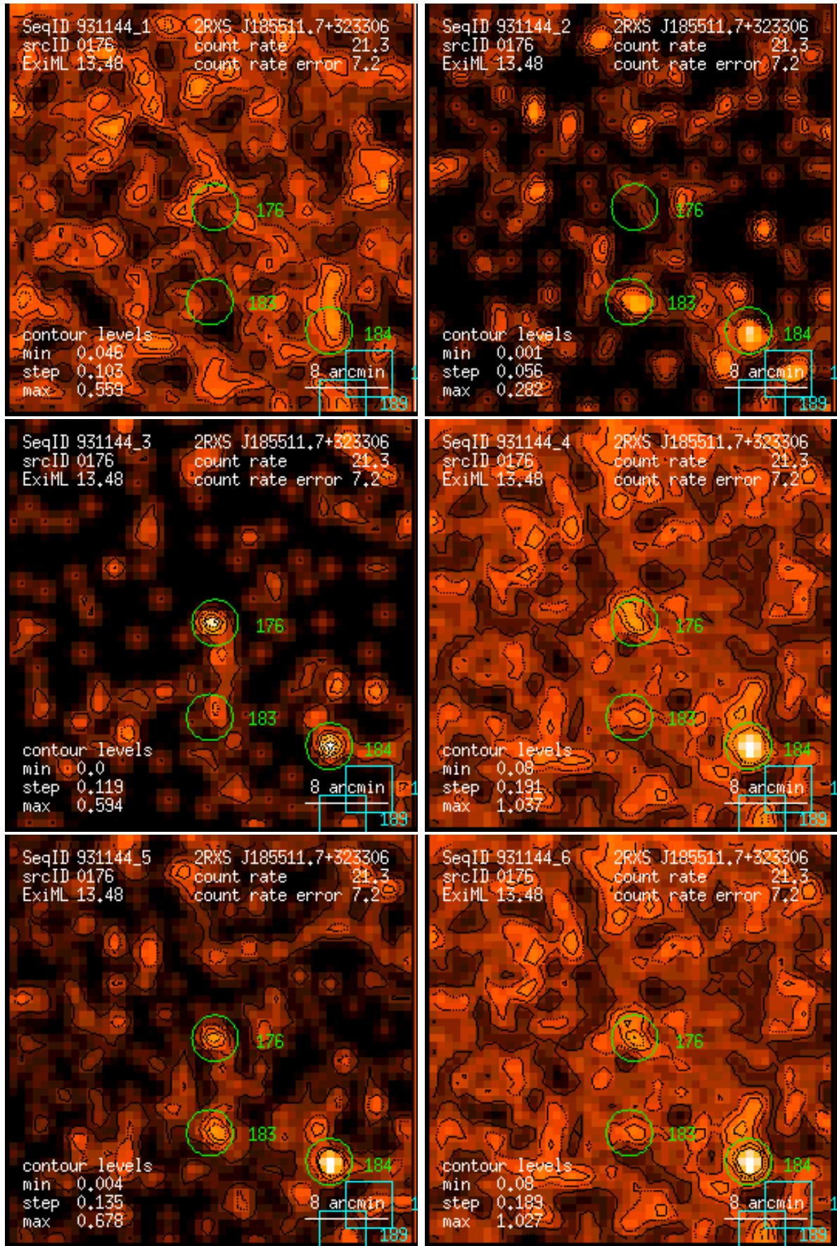
Figure 176: RASS 931144: detection 0176: band rate images, Gaussian filter: (1) PSPC channels 11 – 41, (2) 52 – 90, (3) 91 – 201, (4) 11 – 235, (5) 52 – 201, (6) 11 – 201. Broad band rates in counts/ks. Band rate contour levels in counts/ks/arcmin 2 .
