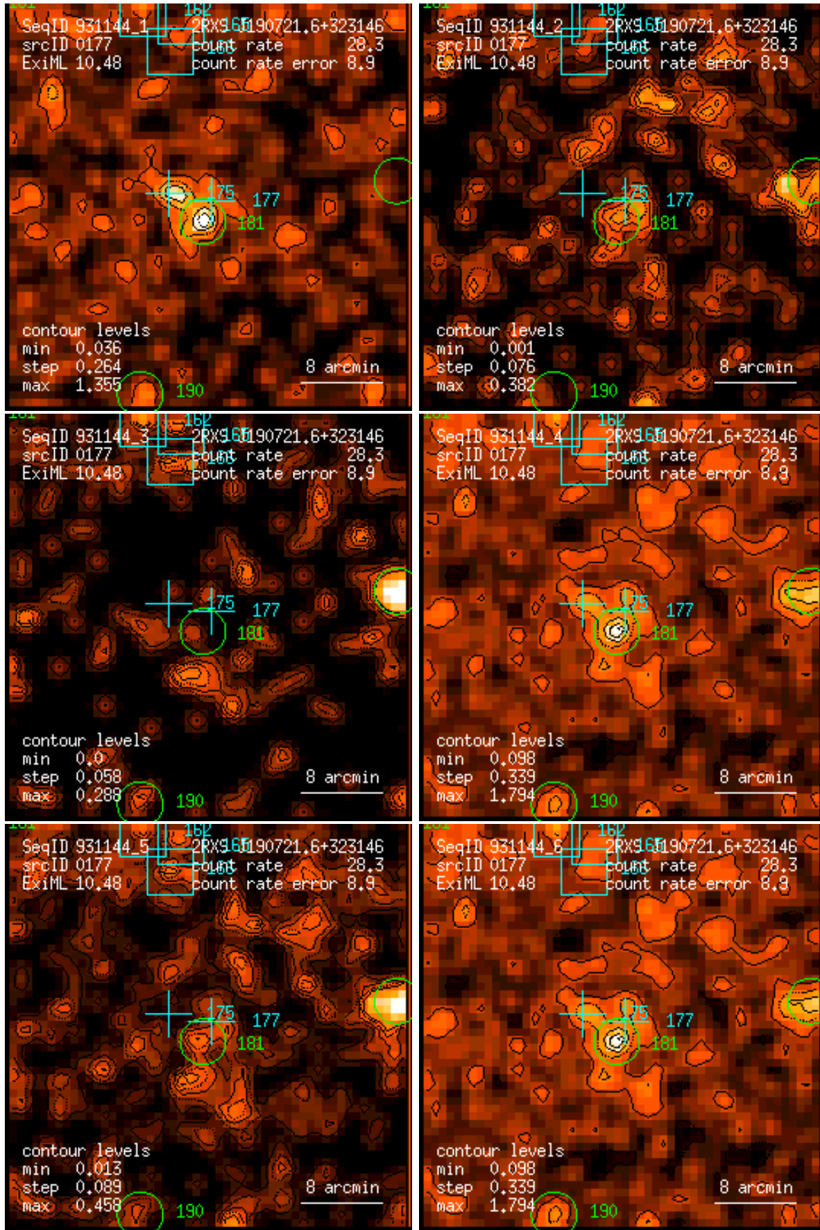
Figure 177: RASS 931144: detection 0177: band rate images, Gaussian filter: (1) PSPC channels 11 – 41, (2) 52 – 90, (3) 91 – 201, (4) 11 – 235, (5) 52 – 201, (6) 11 – 201. Broad band rates in counts/ks. Band rate contour levels in counts/ks/arcmin 2 .
