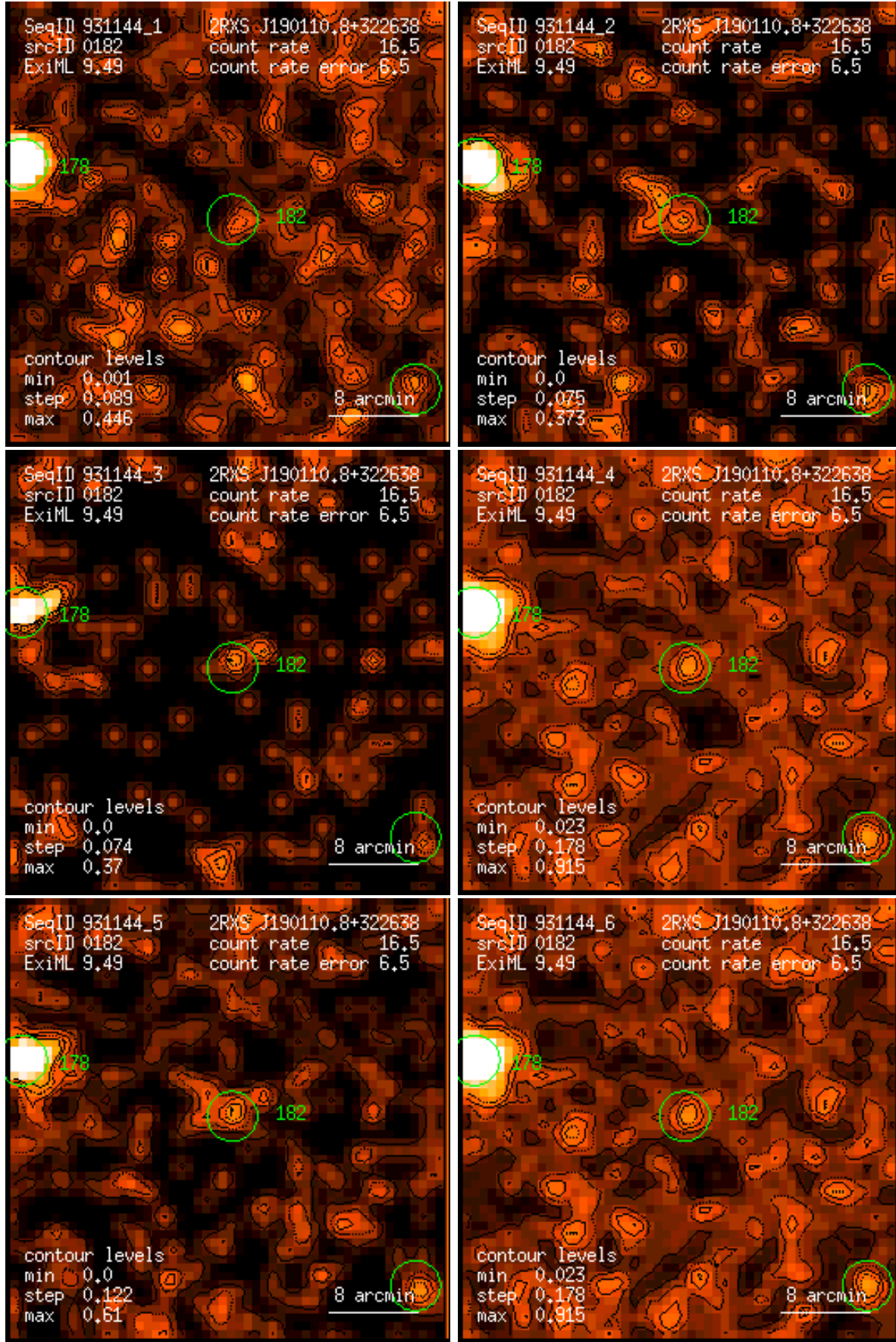
Figure 182: RASS 931144: detection 0182: band rate images, Gaussian filter: (1) PSPC channels 11 – 41, (2) 52 – 90, (3) 91 – 201, (4) 11 – 235, (5) 52 – 201, (6) 11 – 201. Broad band rates in counts/ks. Band rate contour levels in counts/ks/arcmin 2 .
