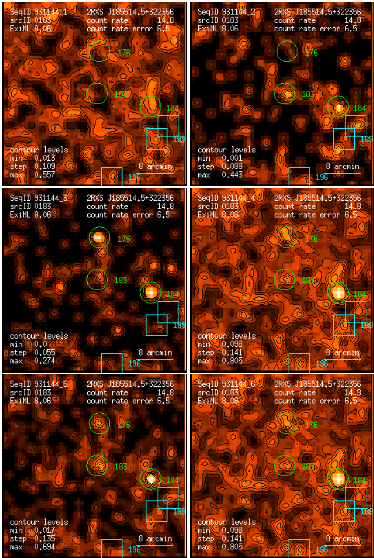
Figure 183: RASS 931144: detection 0183: band rate images, Gaussian filter: (1) PSPC channels 11 – 41, (2) 52 – 90, (3) 91 – 201, (4) 11 – 235, (5) 52 – 201, (6) 11 – 201. Broad band rates in counts/ks. Band rate contour levels in counts/ks/arcmin 2 .
