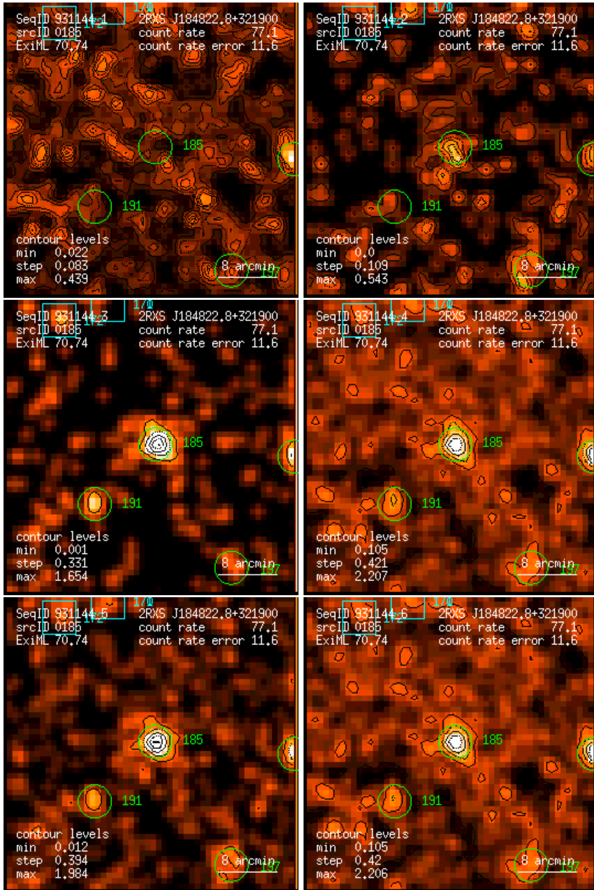
Figure 185: RASS 931144: detection 0185: band rate images, Gaussian filter: (1) PSPC channels 11 – 41, (2) 52 – 90, (3) 91 – 201, (4) 11 – 235, (5) 52 – 201, (6) 11 – 201. Broad band rates in counts/ks. Band rate contour levels in counts/ks/arcmin 2 .
