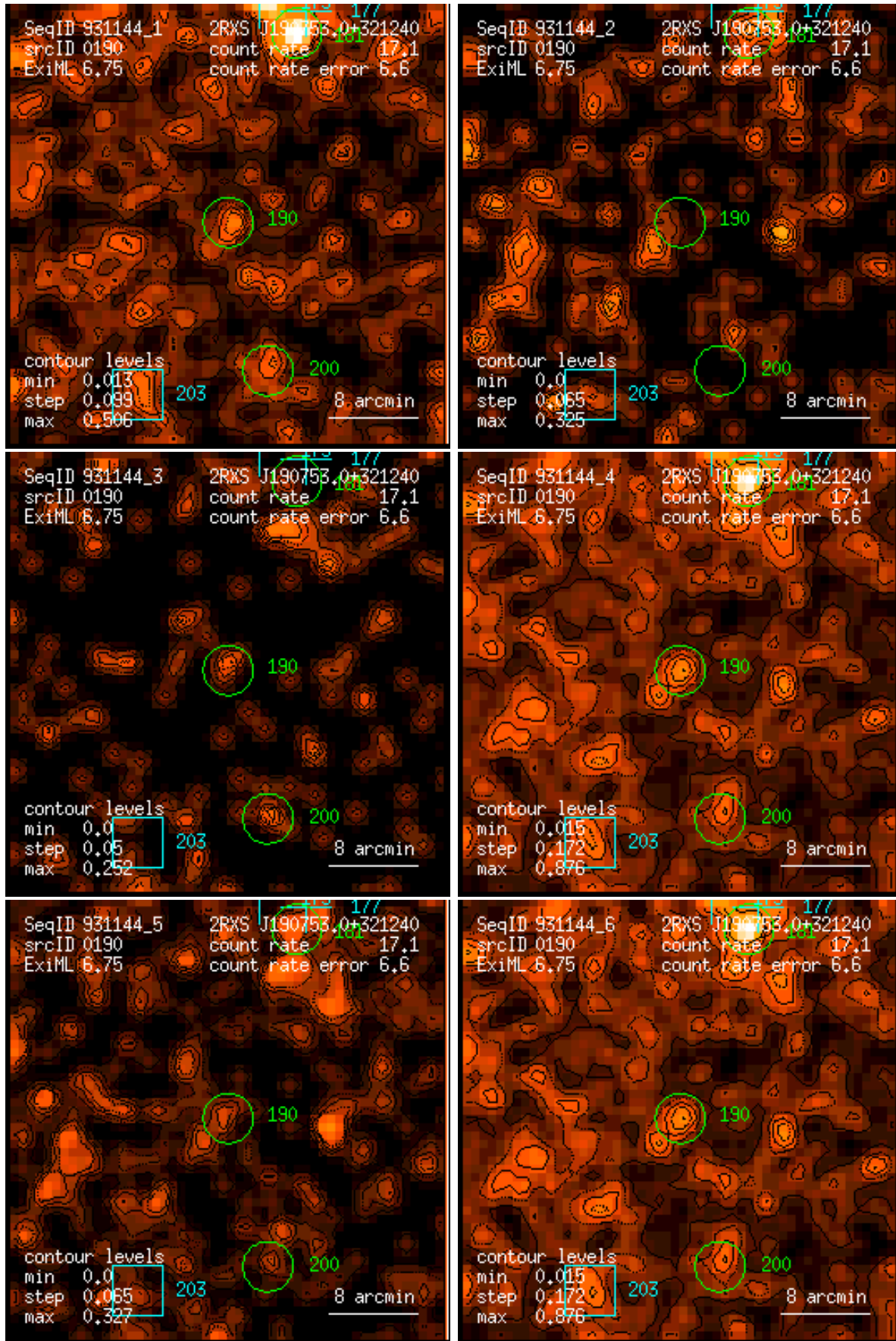
Figure 190: RASS 931144: detection 0190: band rate images, Gaussian filter: (1) PSPC channels 11 – 41, (2) 52 – 90, (3) 91 – 201, (4) 11 – 235, (5) 52 – 201, (6) 11 – 201. Broad band rates in counts/ks. Band rate contour levels in counts/ks/arcmin 2 .
