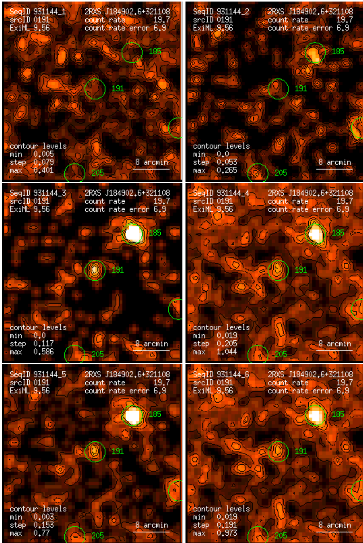
Figure 191: RASS 931144: detection 0191: band rate images, Gaussian filter: (1) PSPC channels 11 – 41, (2) 52 – 90, (3) 91 – 201, (4) 11 – 235, (5) 52 – 201, (6) 11 – 201. Broad band rates in counts/ks. Band rate contour levels in counts/ks/arcmin 2 .
