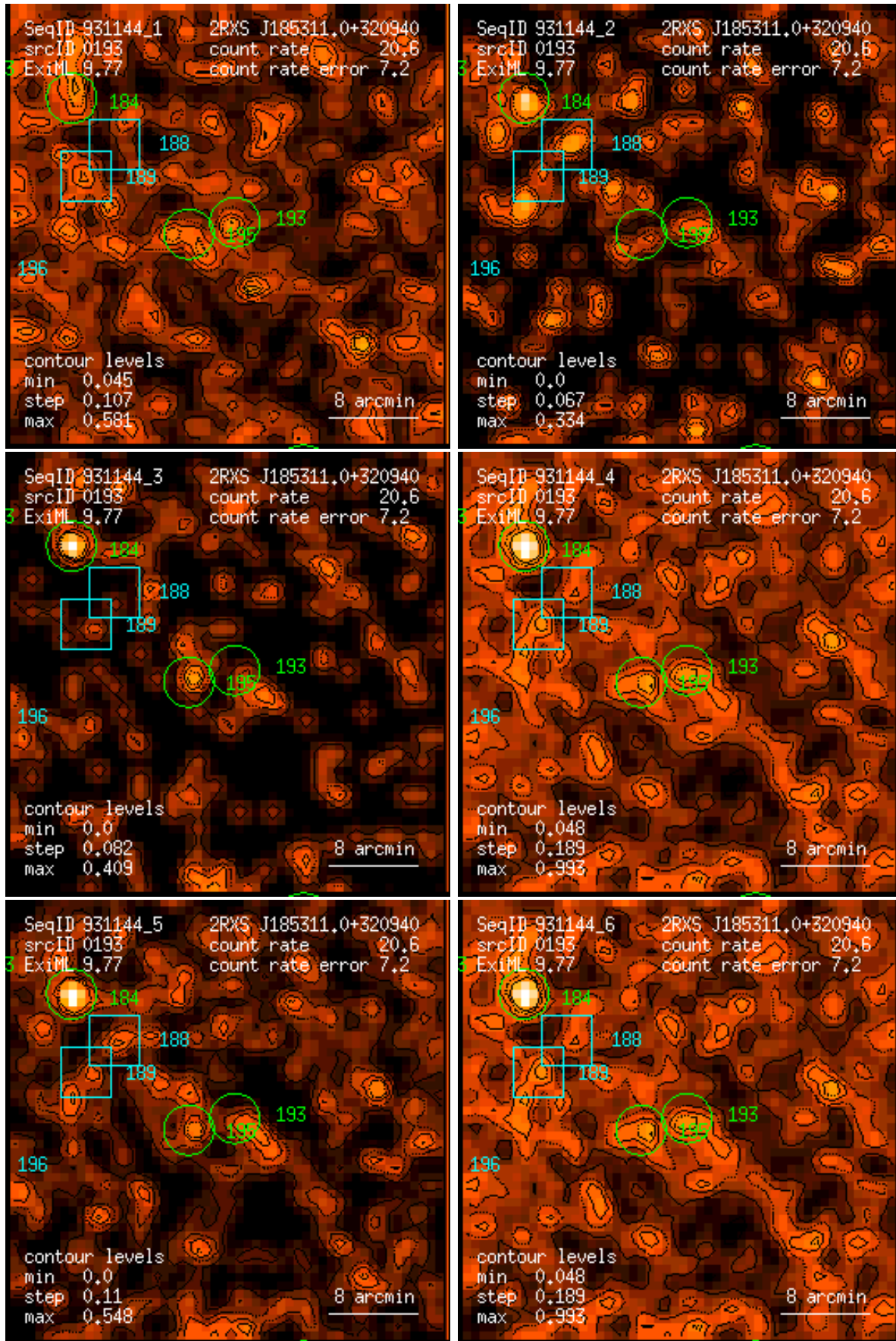
Figure 193: RASS 931144: detection 0193: band rate images, Gaussian filter: (1) PSPC channels 11 – 41, (2) 52 – 90, (3) 91 – 201, (4) 11 – 235, (5) 52 – 201, (6) 11 – 201. Broad band rates in counts/ks. Band rate contour levels in counts/ks/arcmin 2 .
